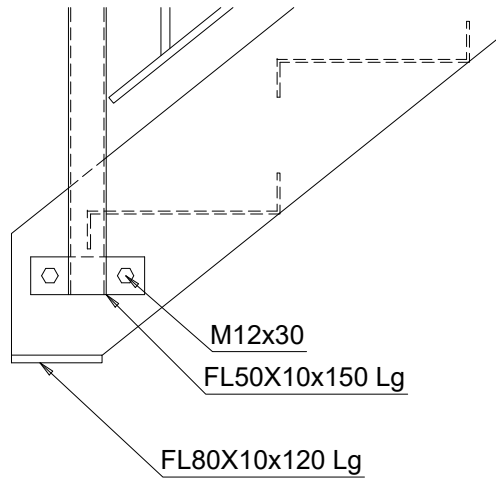
DETAIL-C
