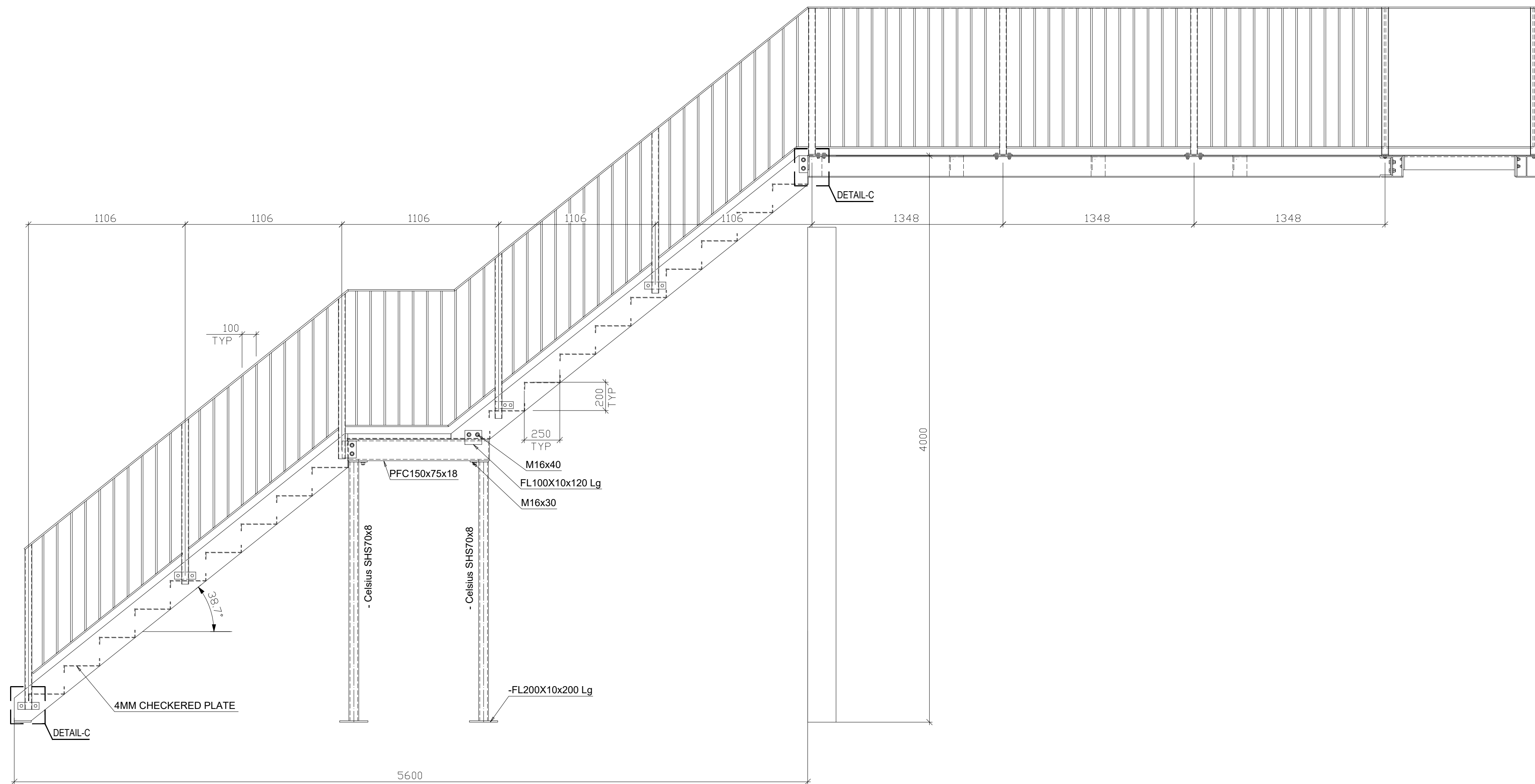
ELEVATION-1
