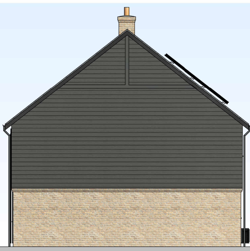
Proposed Side Elevation 2 1 : 100
