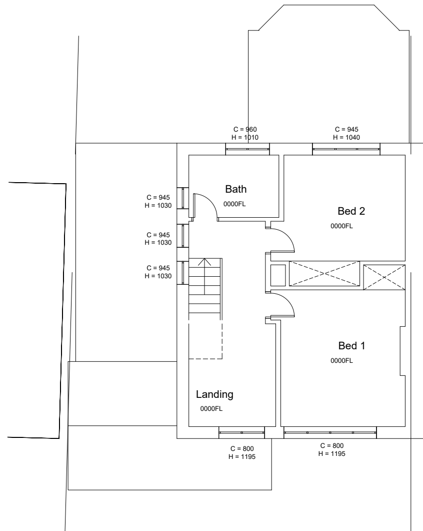
First Floor 1:100
