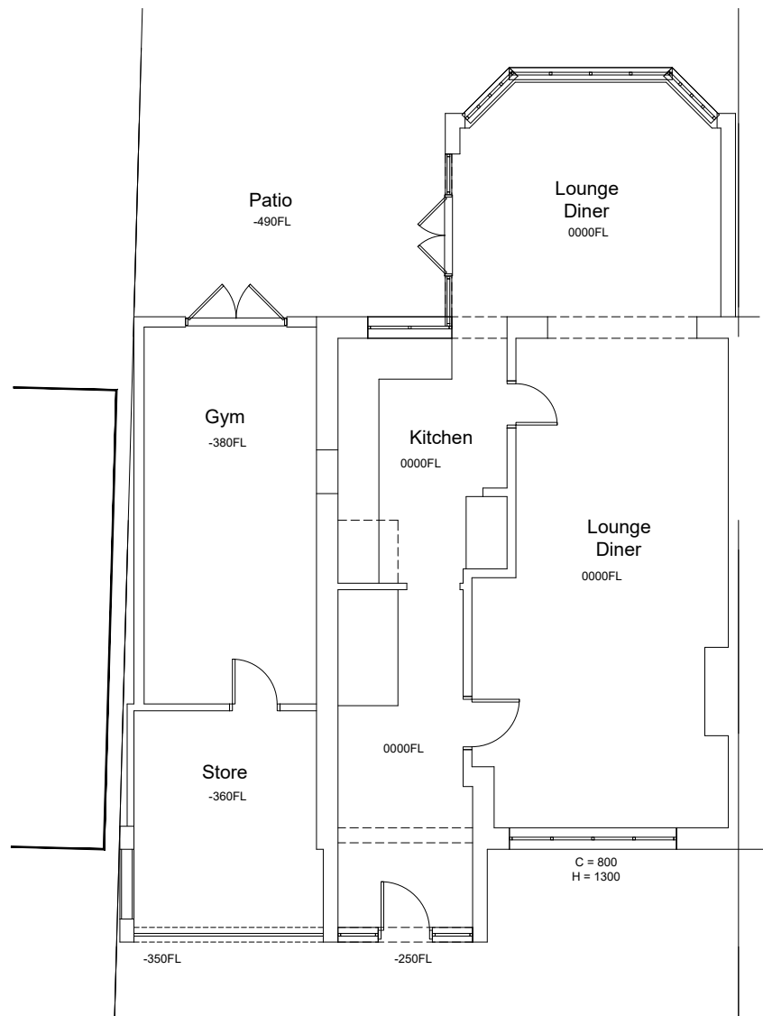
Ground Floor 1:100
