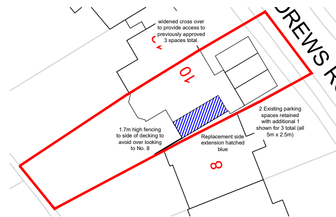
Proposed Block Plan 1:500
