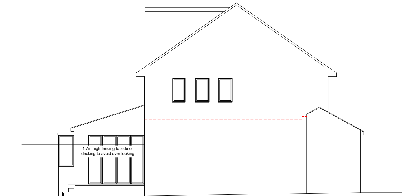
Proposed Side Elevation (SE) 1:100
