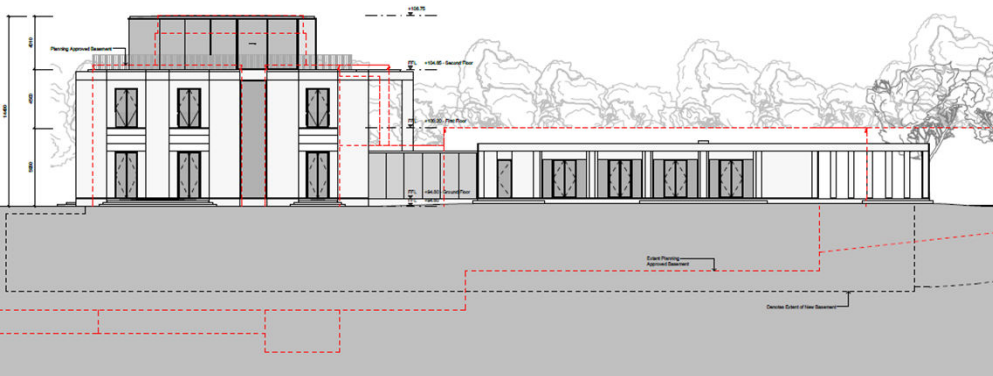
PCY-PBC-MH-ZZ-DR-A-1021 (E Elev)
