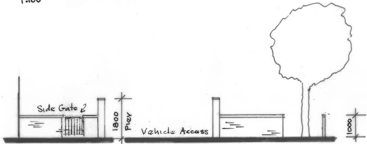
Side Elevation (Wall rebuilt on existing foundations)
