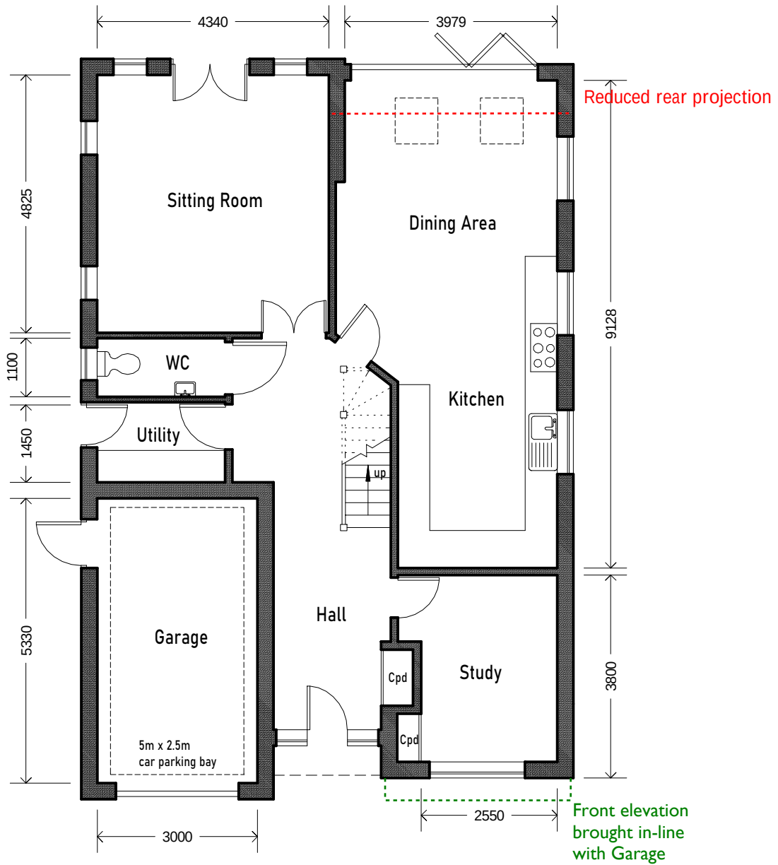
GROUND FLOOR
