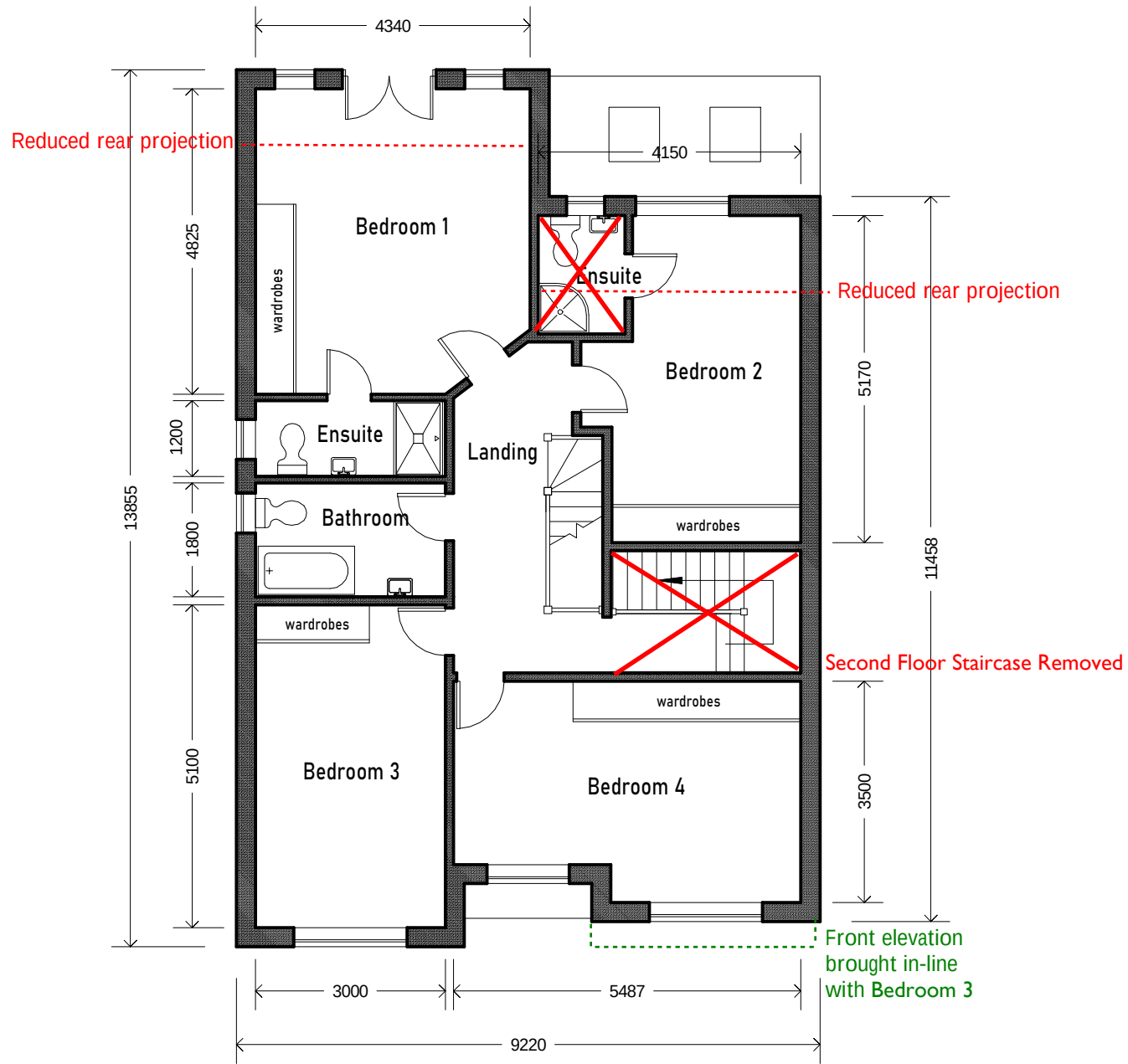
FIRST FLOOR
