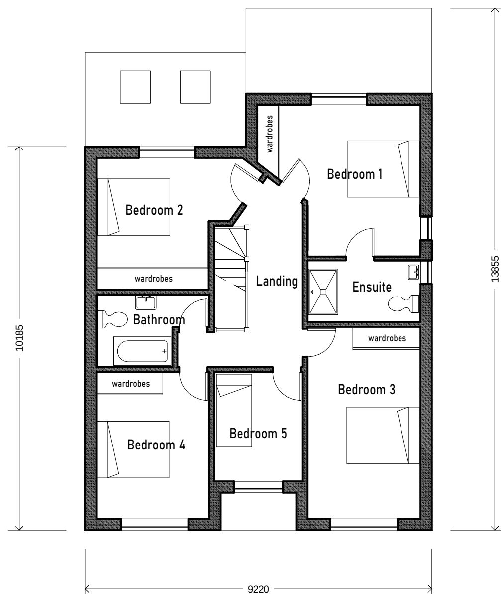
FIRST FLOOR
