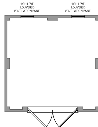
FLOOR PLAN
