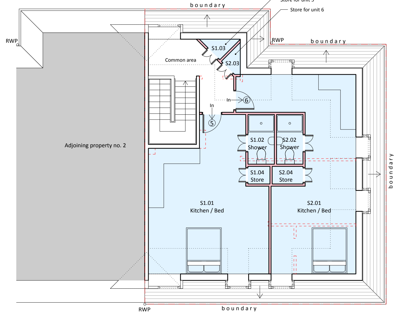
3 SECOND Scale: 1:100 UNIT 5 & 6
