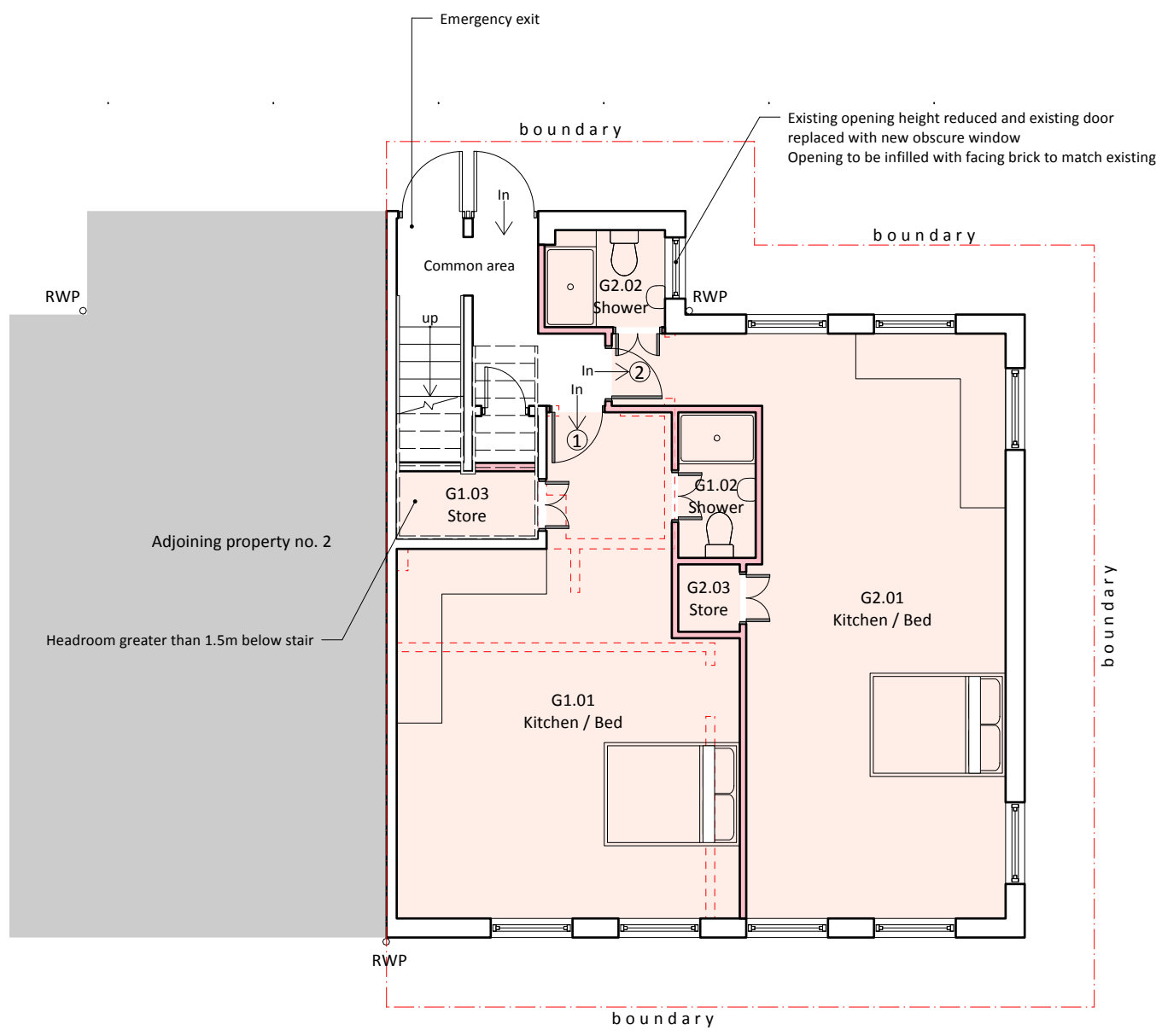
1 GROUND Scale: 1:100 UNIT 1 & 2
