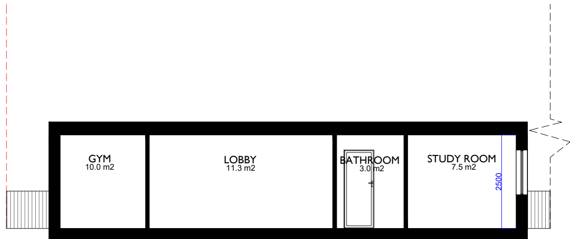
Existing AA Section
