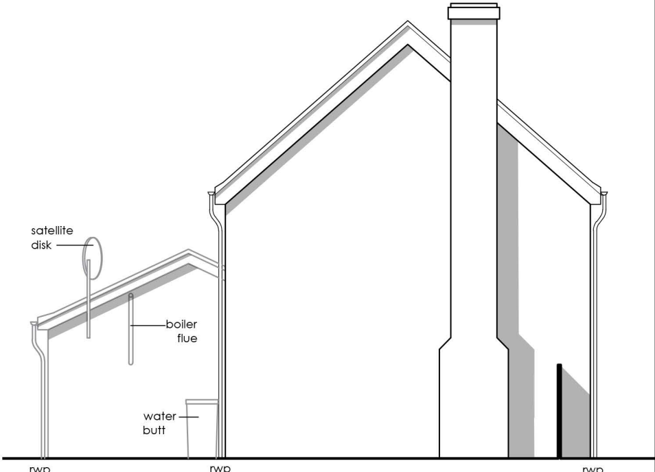
EXISTING WEST (SIDE) ELEVATION 1/100
