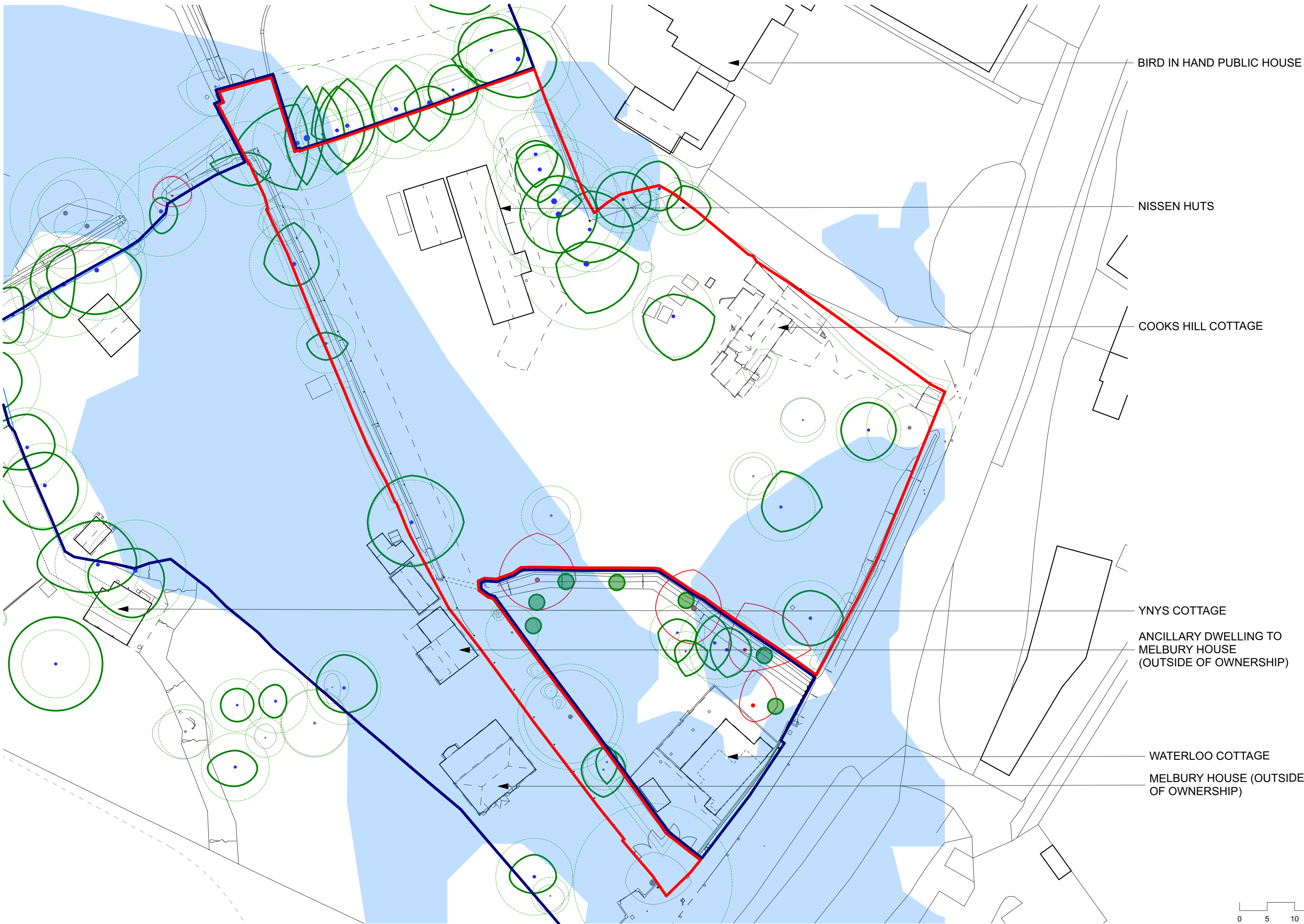
SITE CONSTRAINTS PLAN
