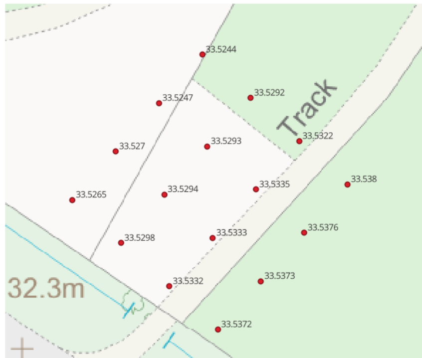
Figure 7: 1 in 100y+35% flood levels, mAOB
