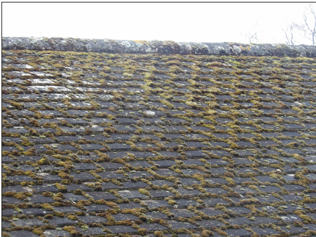
Figure 4. Example of roof and ridge tiles. Orchard Cottage, Hurst. 18.03.25
