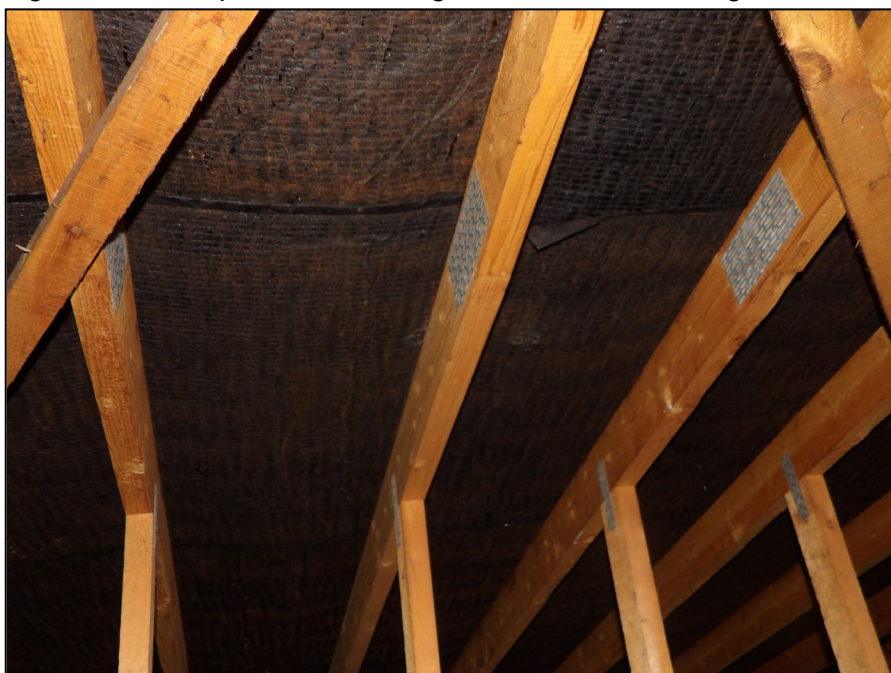
Figure 11. Example bitumen lining in loft. Orchard Cottage, Hurst. 28.03.25
