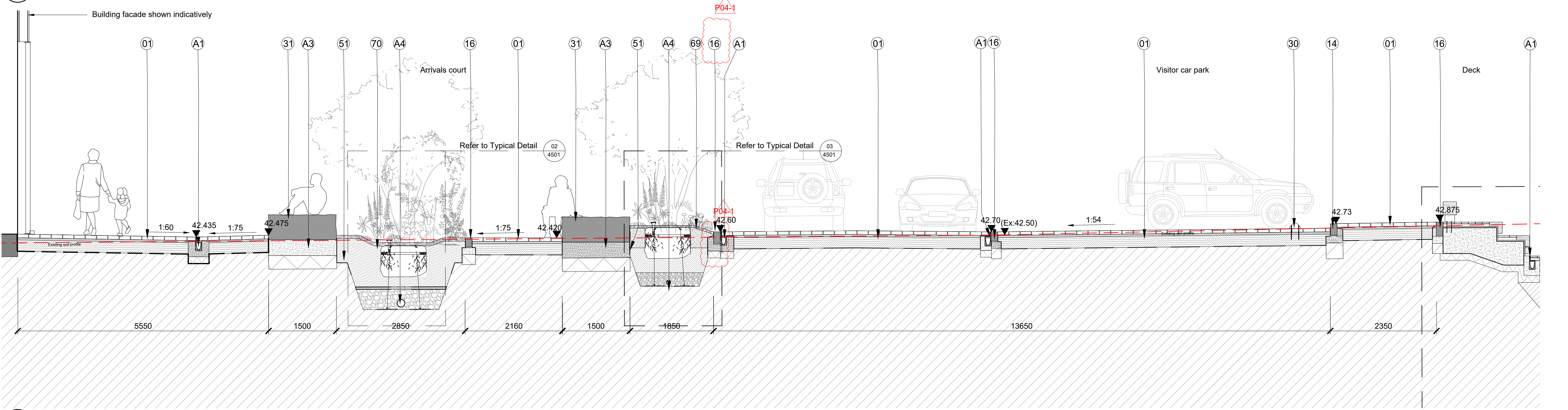
02 Section 1 - A scale 1:50 @ A1
