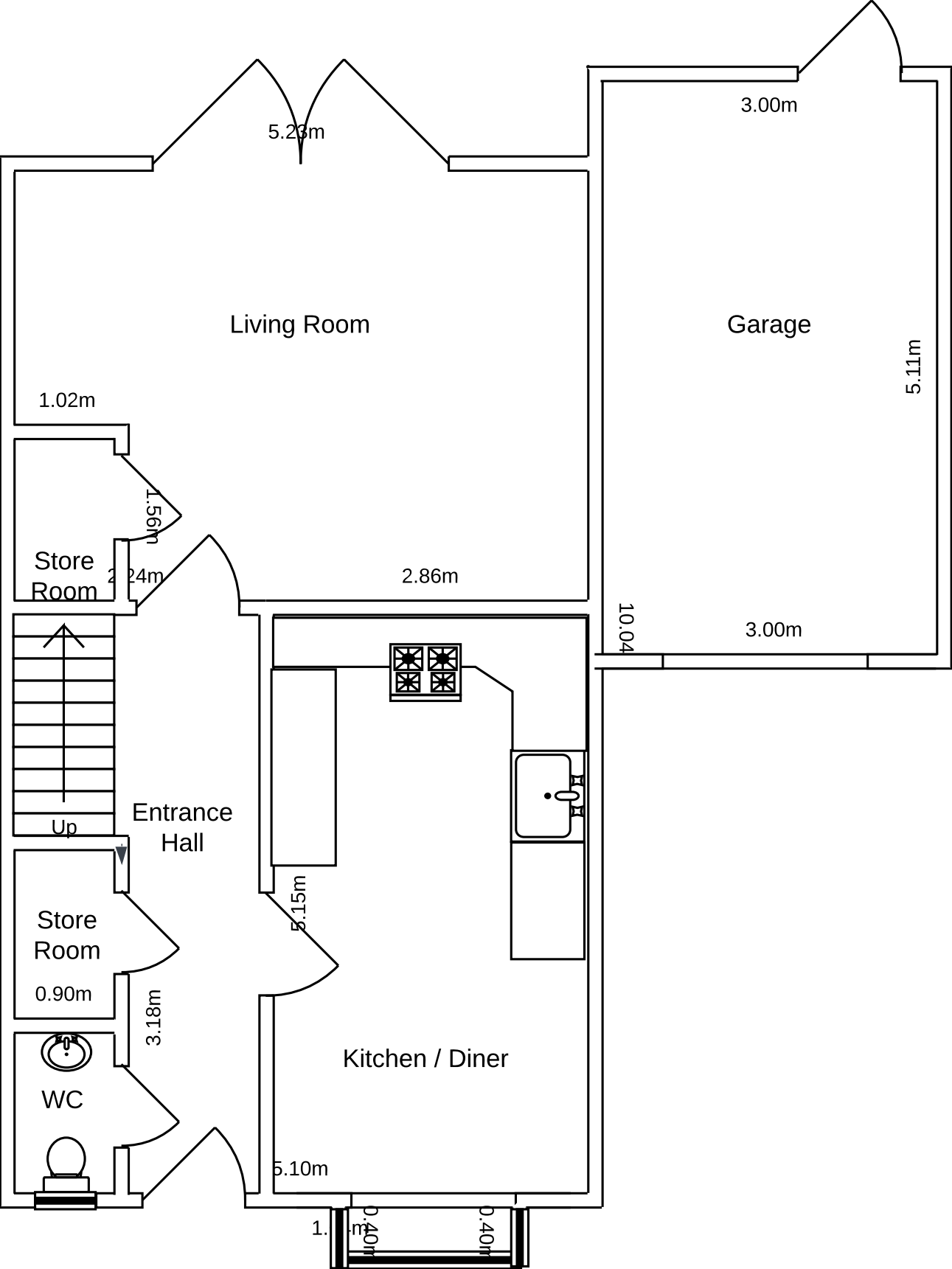
18 Priors Gardens - Ground Floor Plan
