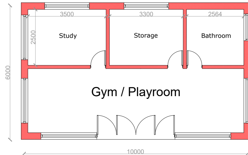
Proposed floorplan
