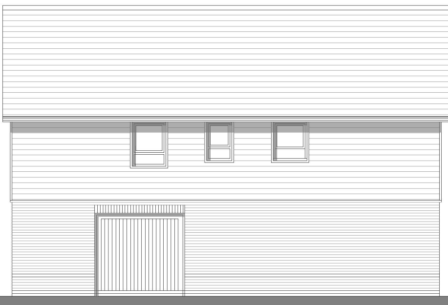
Rear Elevation
