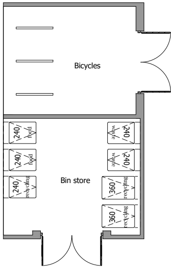
Ground Floor Plan Plots 86-91 , handed for plots 92-97
