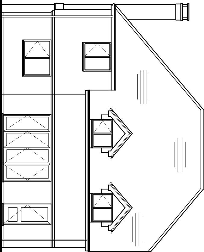
REAR ELEVATION
