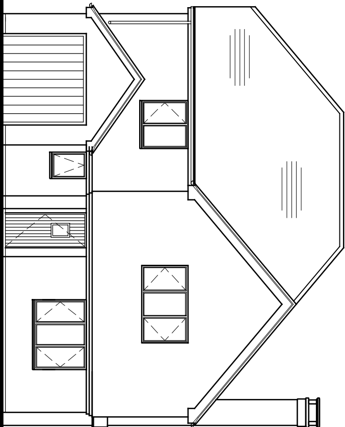
FRONT ELEVATION
