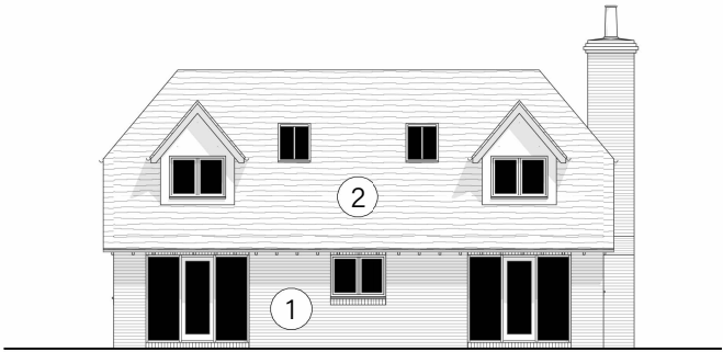
SOUTH ELEVATION
