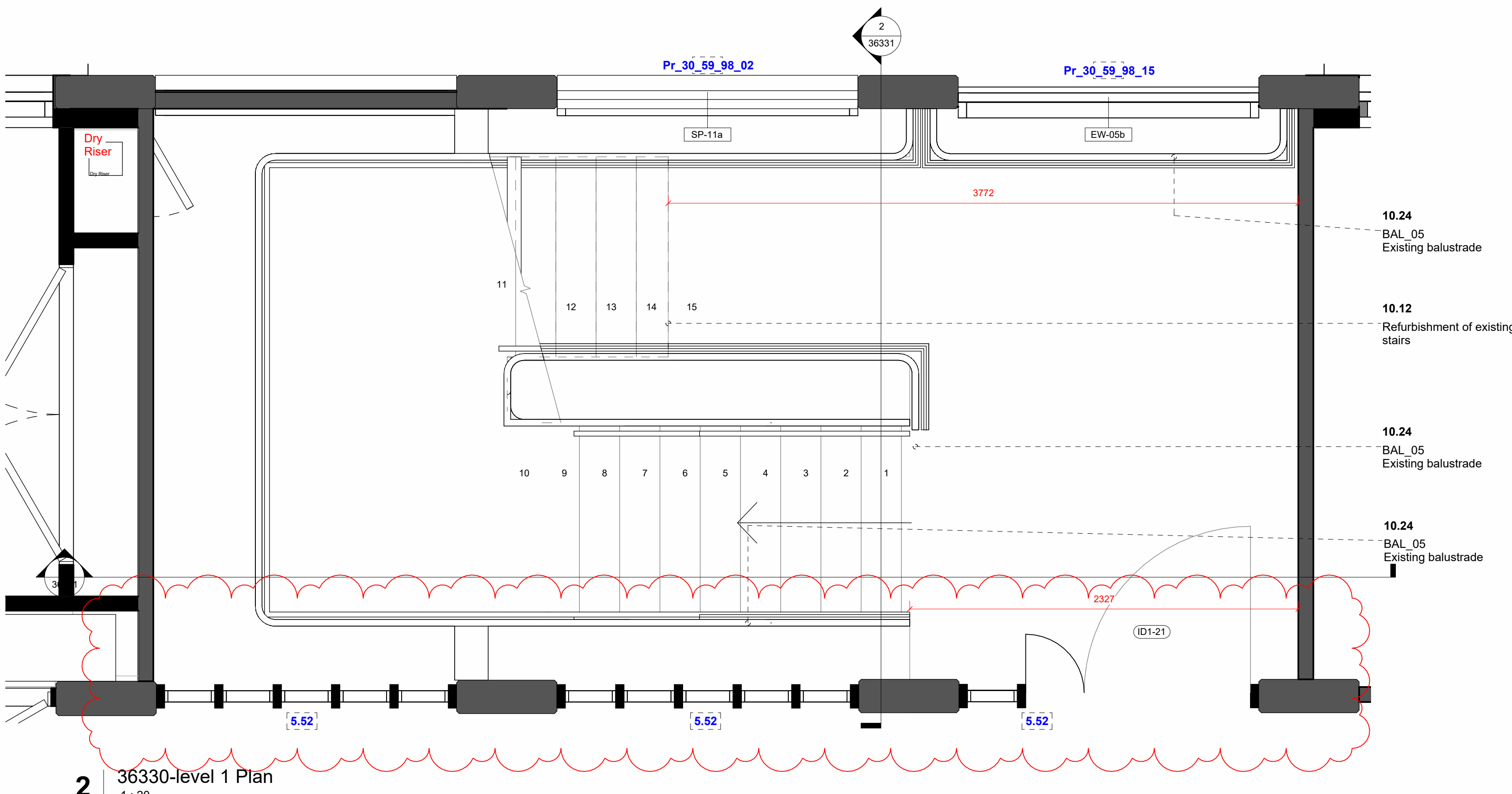
2 | 36330-level 1 Plan 1 : 20
