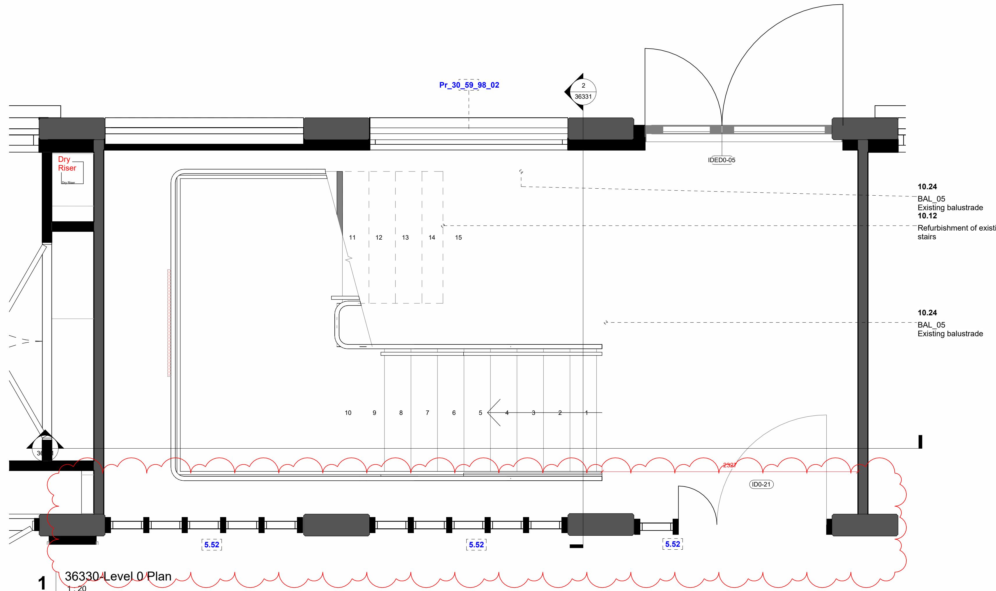
1 | 36330-Level 0 Plan 1 : 20
