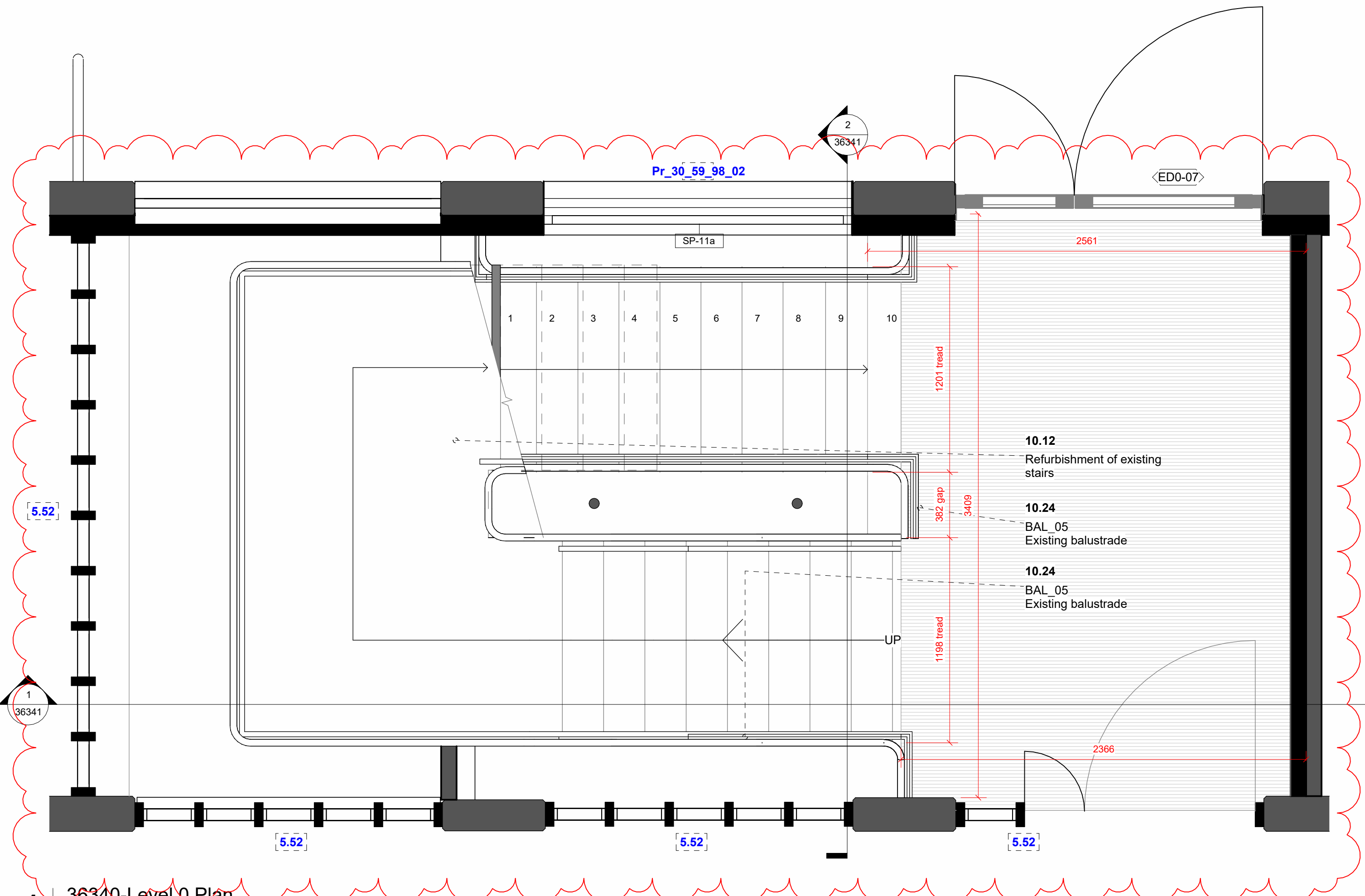
1 36340-Level 0 Plan 1:20
