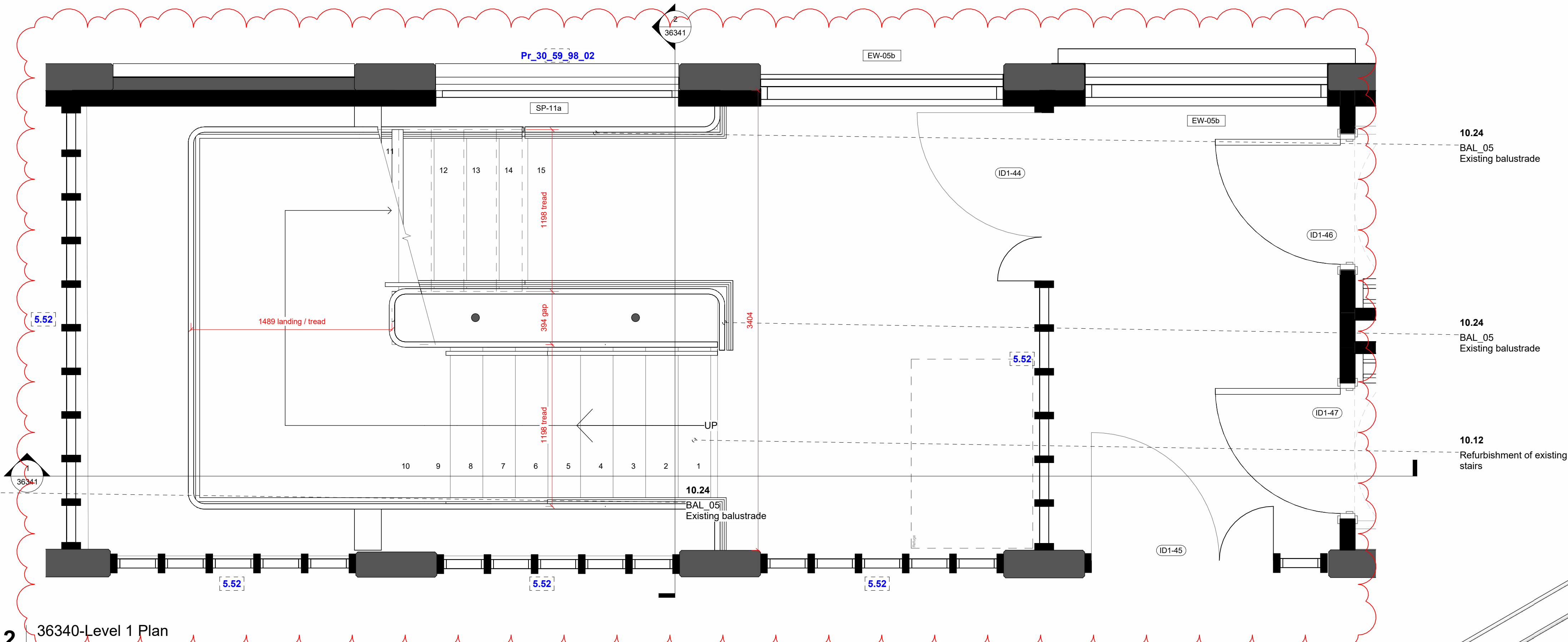
2 36340-Level 1 Plan 1:20
