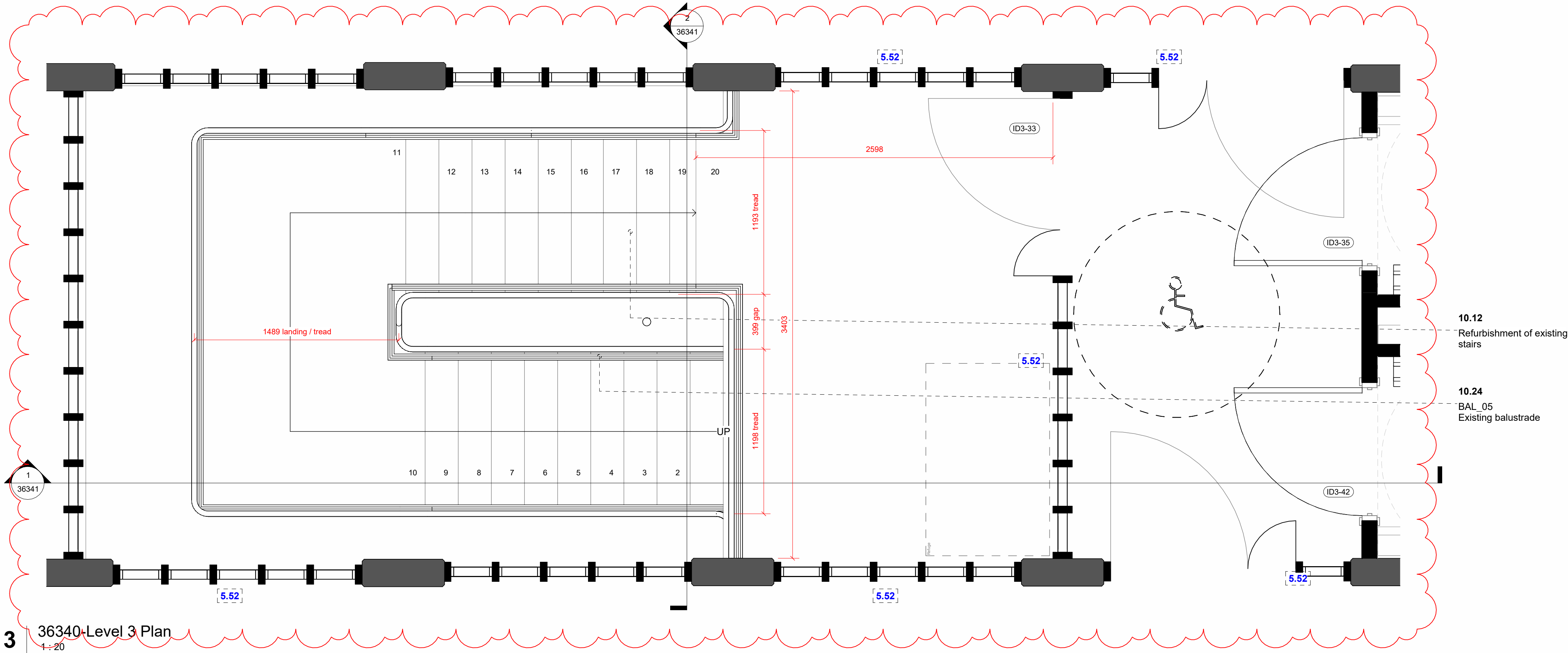
3 36340-Level 3 Plan 1:20
