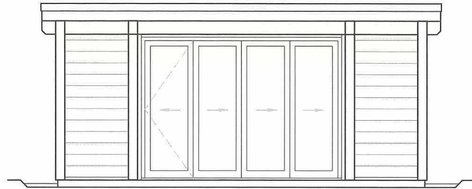
Front Elevation (NORTH)
