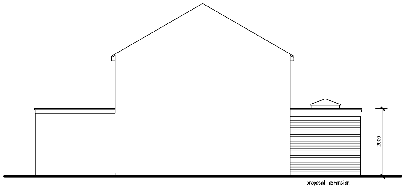
SIDE ELEVATION
