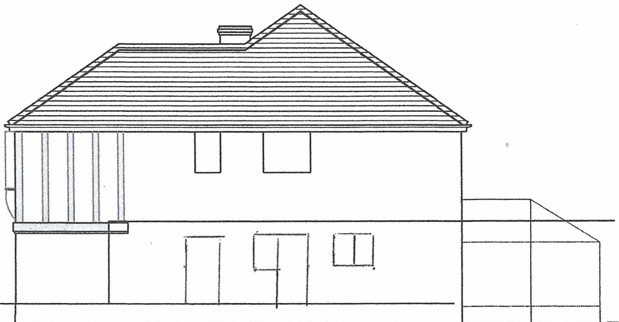
Side elevation (existing) (no changes)
