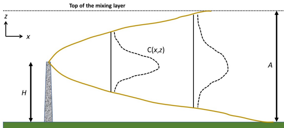
Figure A.1: Vertical Cross-section through a Plume
