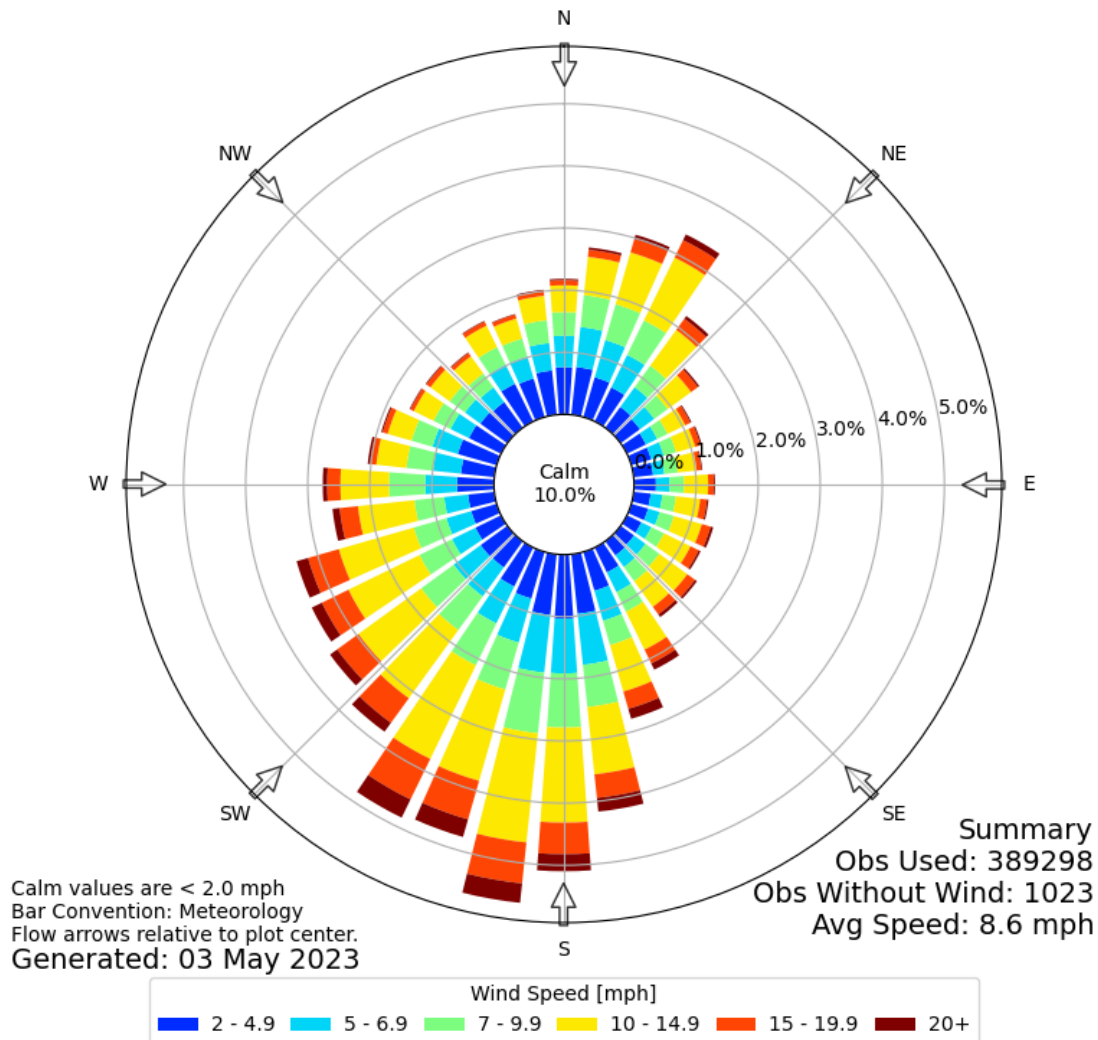
Figure 3: Windrose for RAF Benson (Benson, Ewelme, Wallingford OX10 6AA). The lengths of the bars show the frequency with which the wind blows from each sector and the colours show the contributions from different intervals of wind speed. Circular contours are at frequency intervals of 1%. From the Iowa Environmental Mesonet of Iowa State University. 7 Downloaded 10 July 2023.
