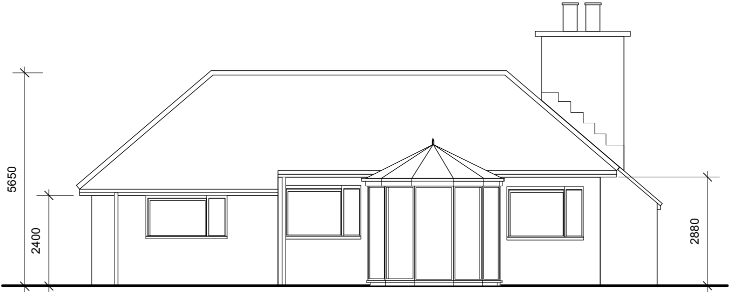
REAR/SOUTH ELEVATION
