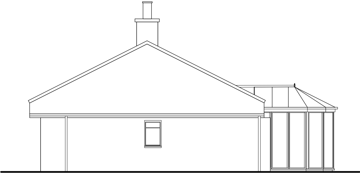
SIDE/WEST ELEVATION
