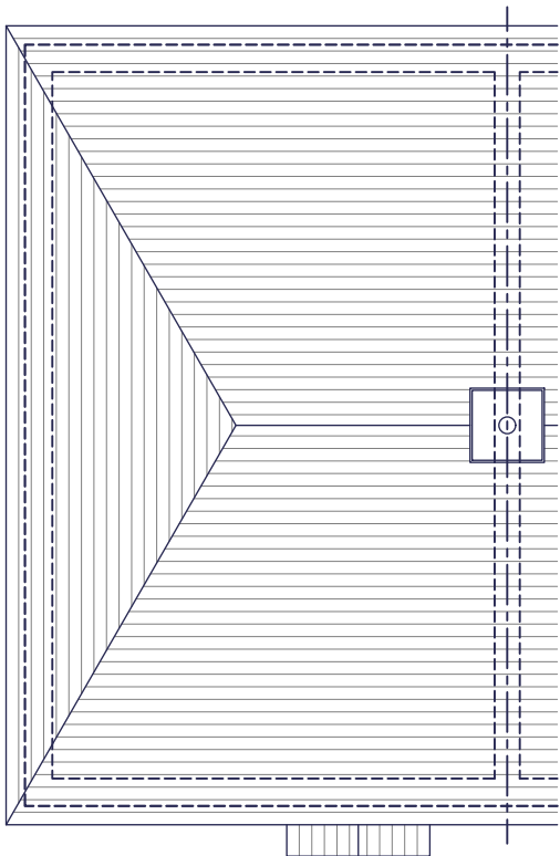
ROOF PLAN
