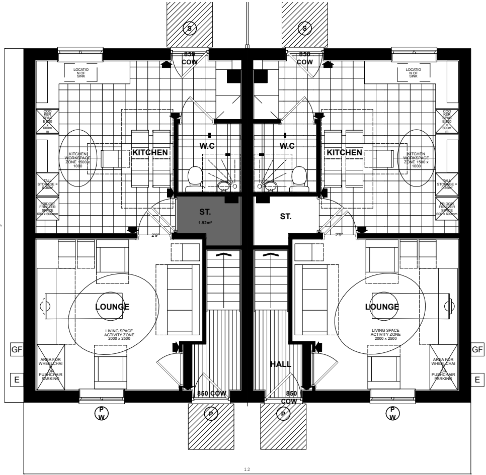
NSS.M3B5P GROUND FLOOR PLAN
