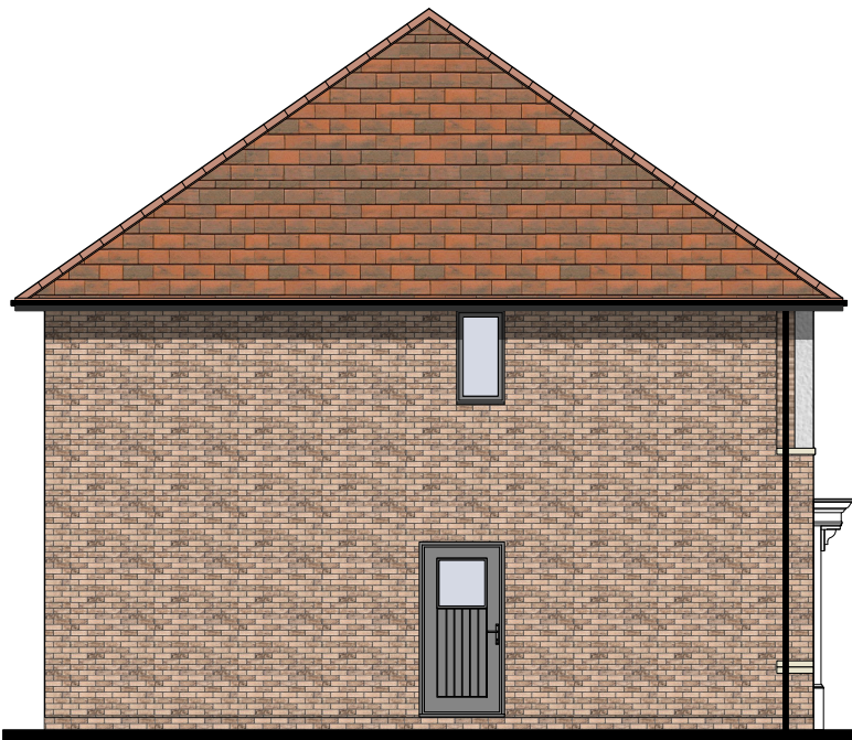
SIDE ELEVATION
