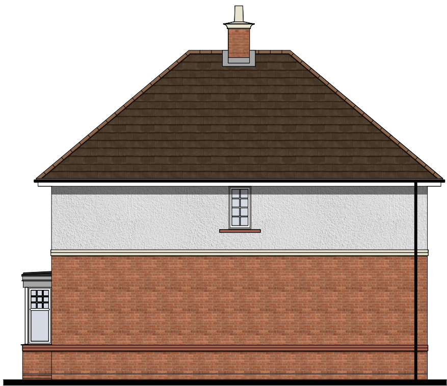
CLA412 REAR ELEVATION
