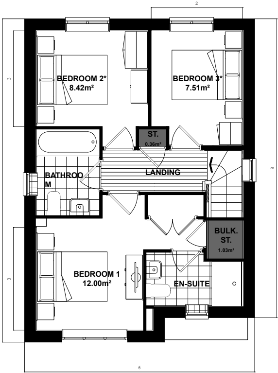
NSS.382 FIRST FLOOR PLAN
