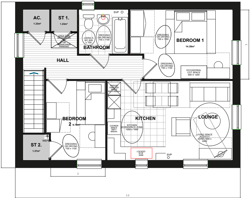
2BF03 FIRST FLOOR PLAN
