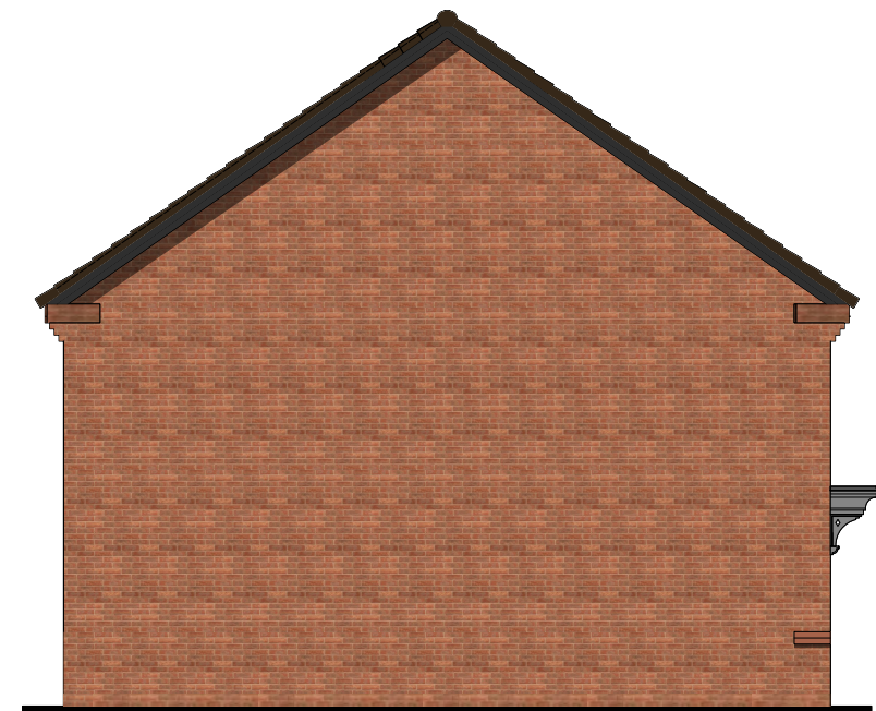
NSS.3B5P SIDE ELEVATION
