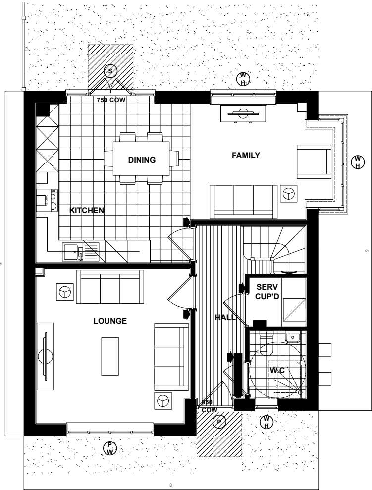
M401 GROUND FLOOR PLAN
