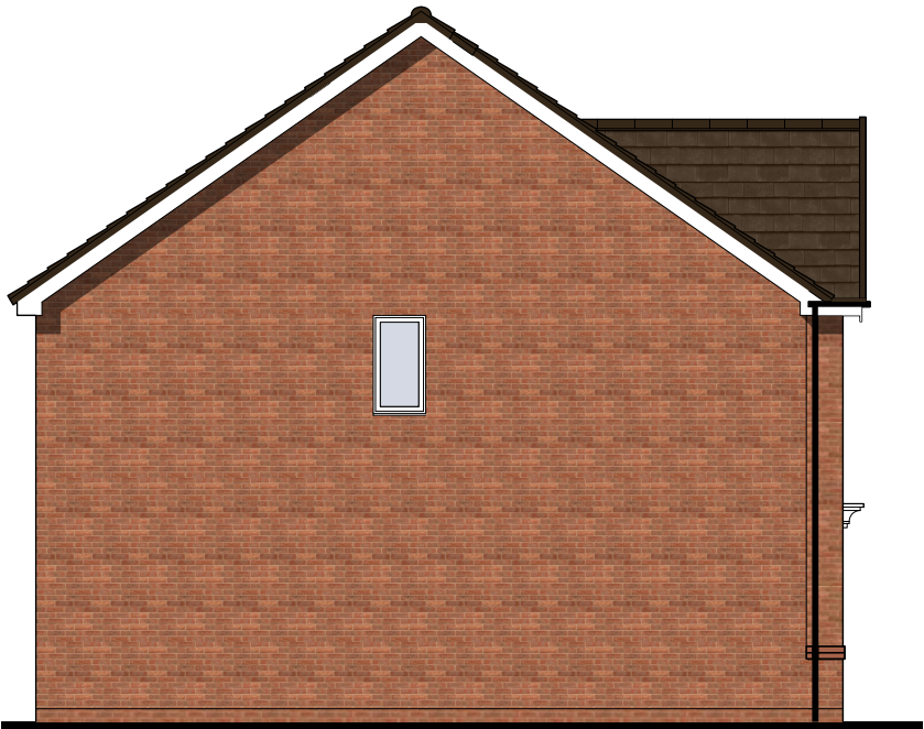
NSS.378 KANE SIDE ELEVATION
