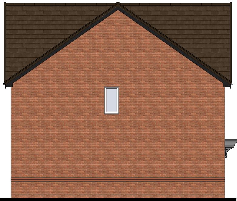
NSS.372 BUXTON SIDE ELEVATION
