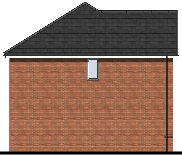
NSS.382 SIDE ELEVATION
