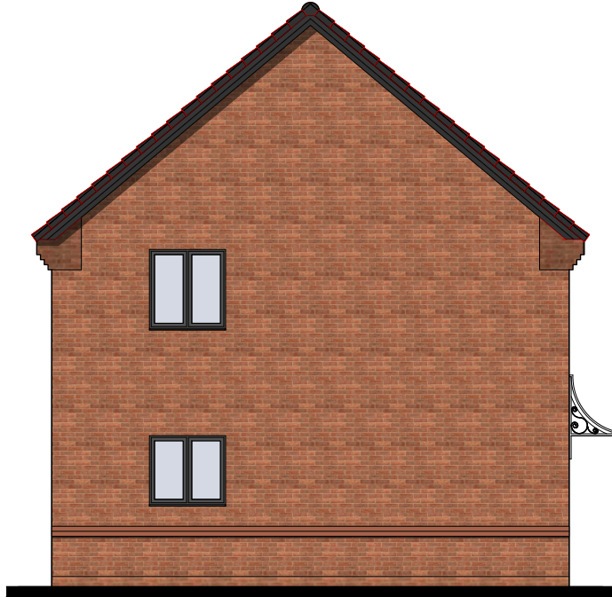
SIDE ELEVATION
