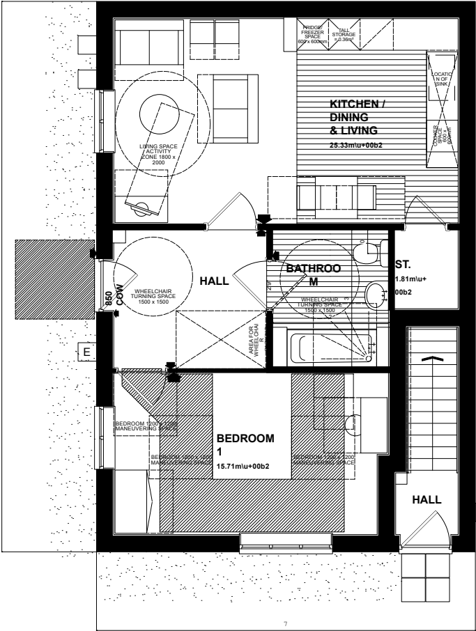
M4(3)1BF01 GROUND FLOOR PLAN
