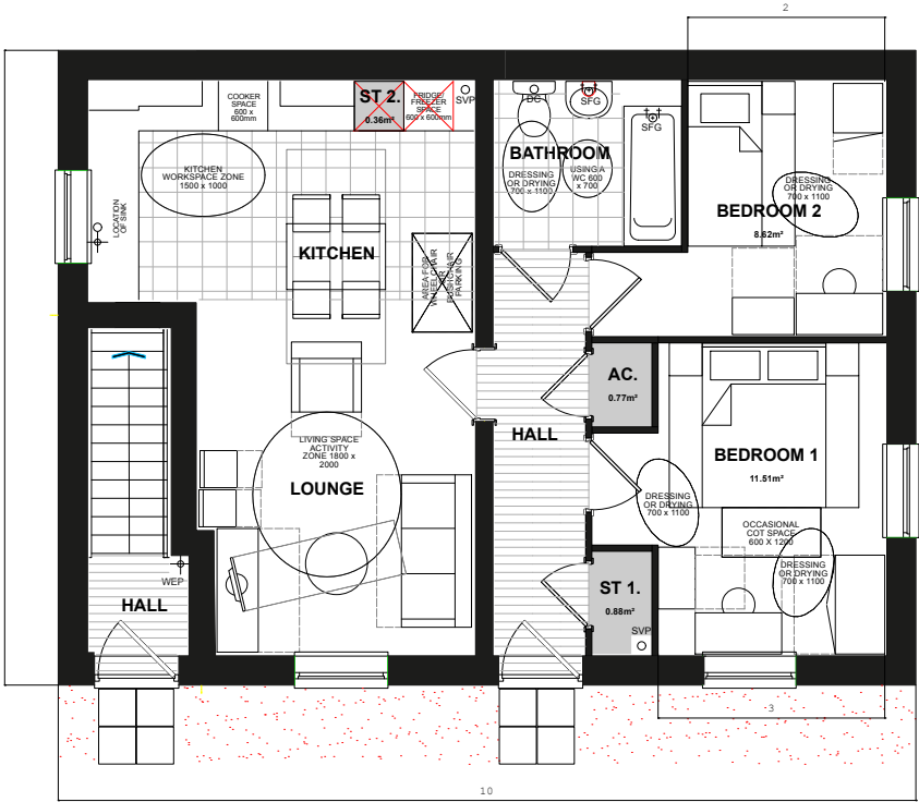
2BF03 GROUND FLOOR PLAN
