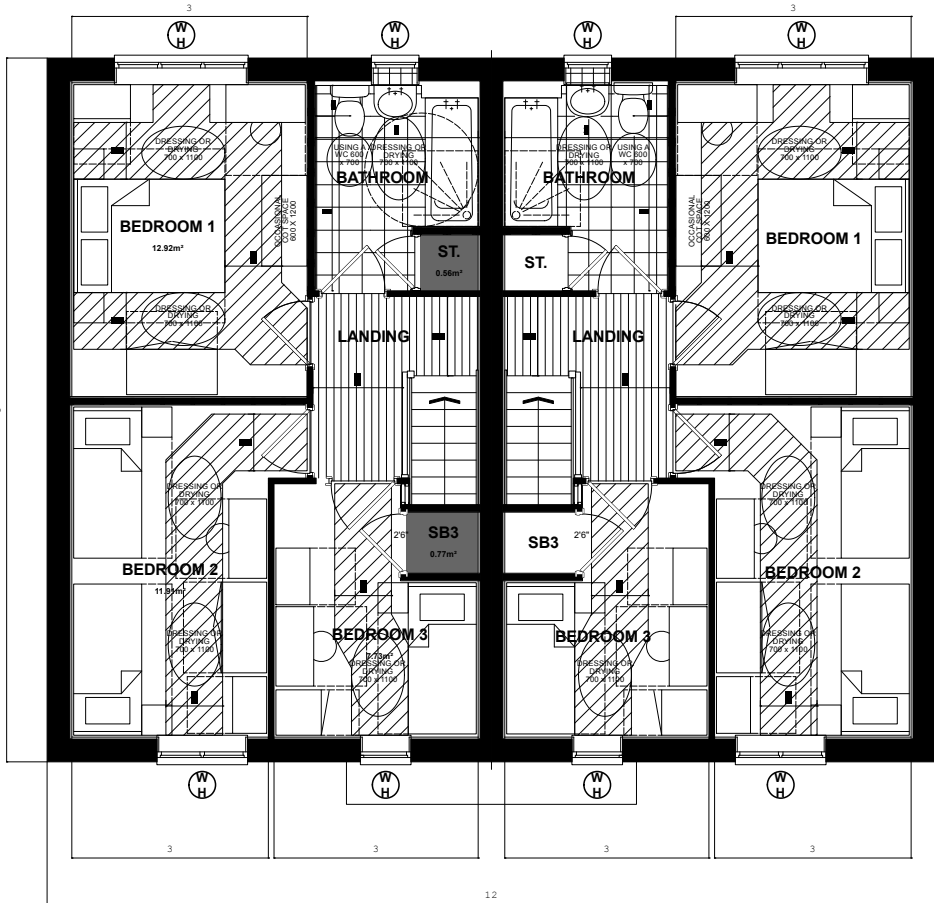
NSS.M3B5P FIRST FLOOR PLAN
