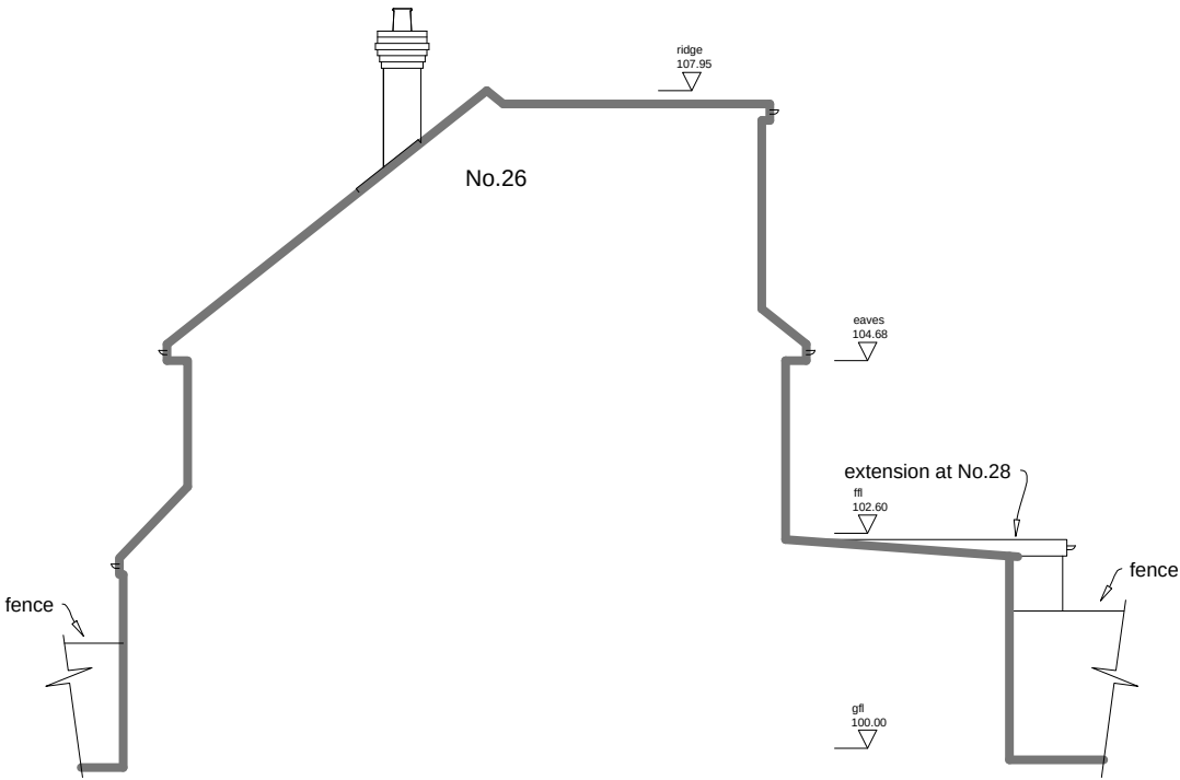
SOUTH WEST (SIDE) ELEVATION
