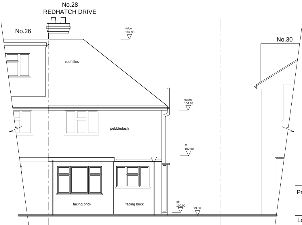
SOUTH EAST ( REAR ) ELEVATION
