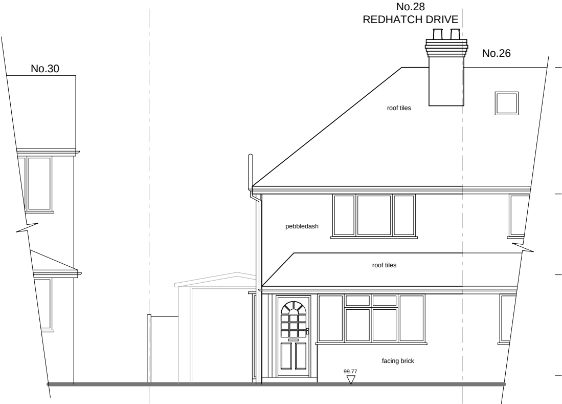
NORTH WEST ( FRONT) ELEVATION
