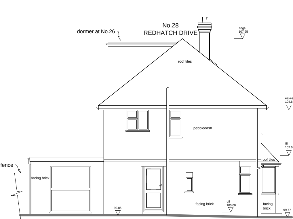
NORTH EAST ( SIDE ) ELEVATION
