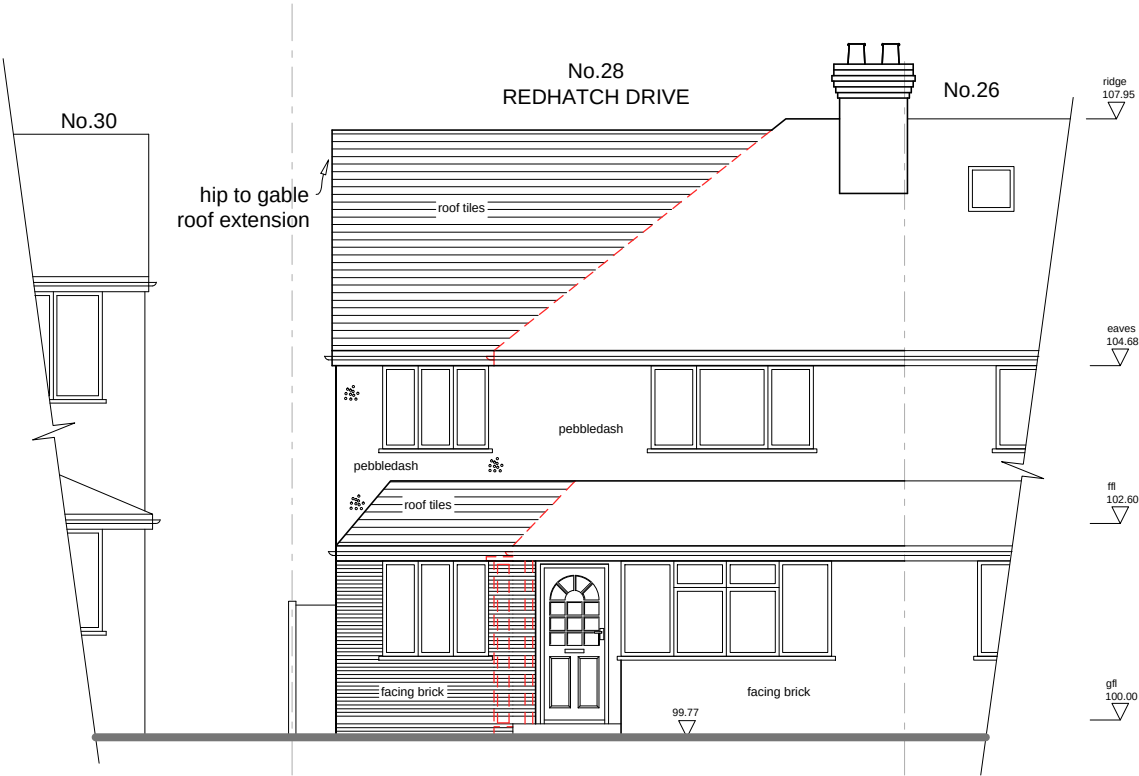
NORTH WEST ( FRONT ) ELEVATION
