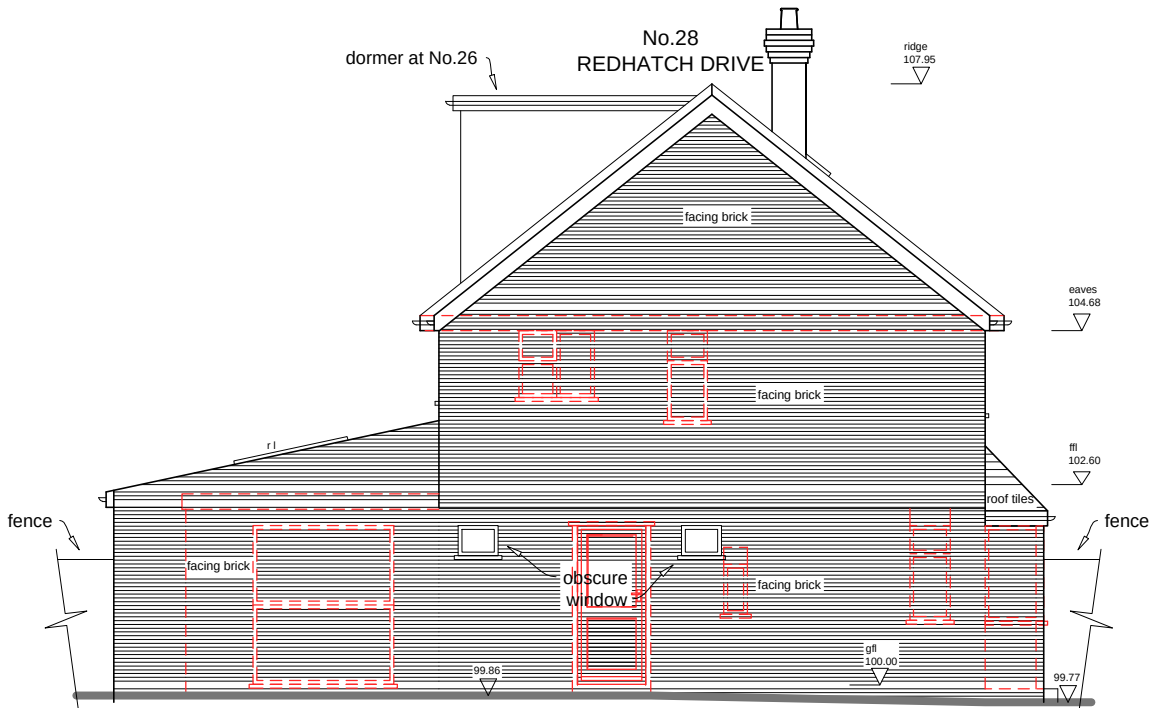
NORTH EAST ( SIDE ) ELEVATION
