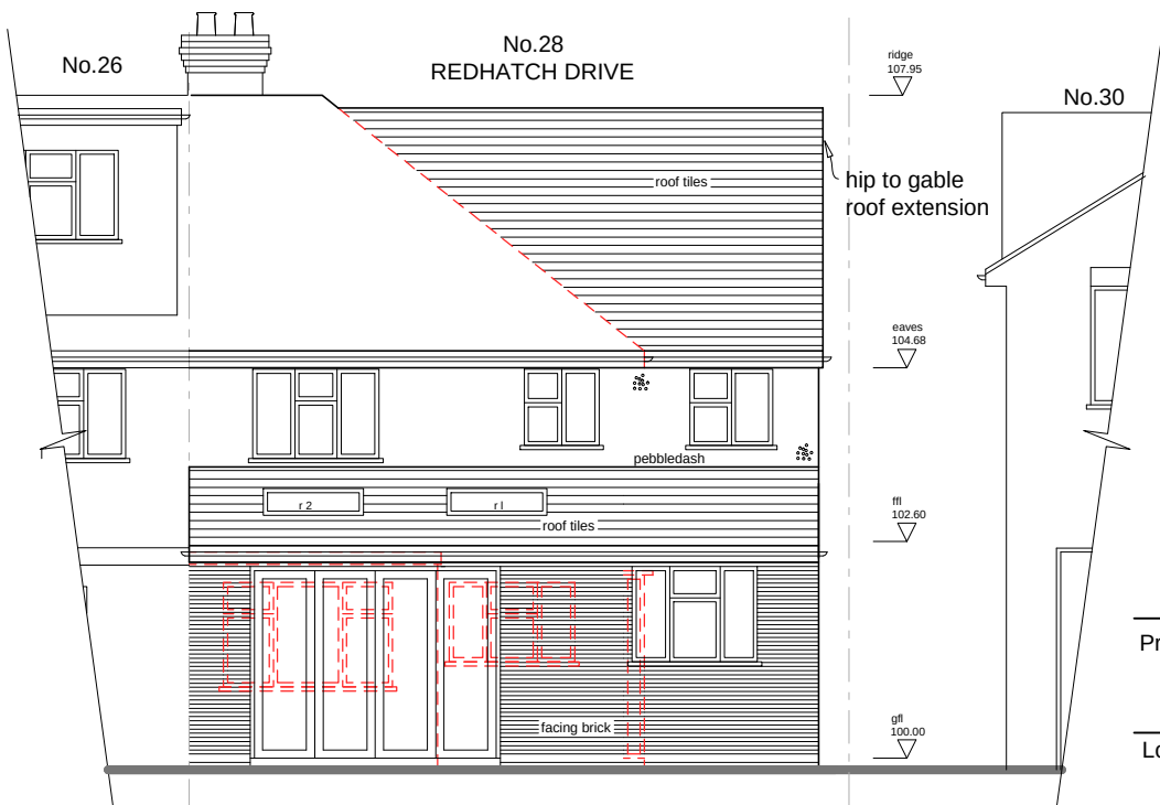
SOUTH EAST ( REAR ) ELEVATION
