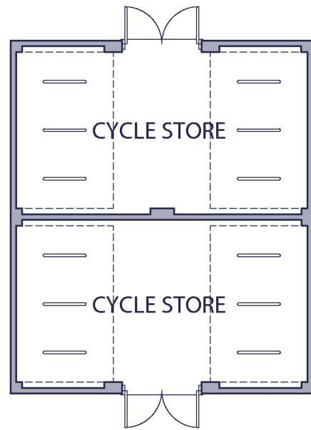
FLOOR PLAN
