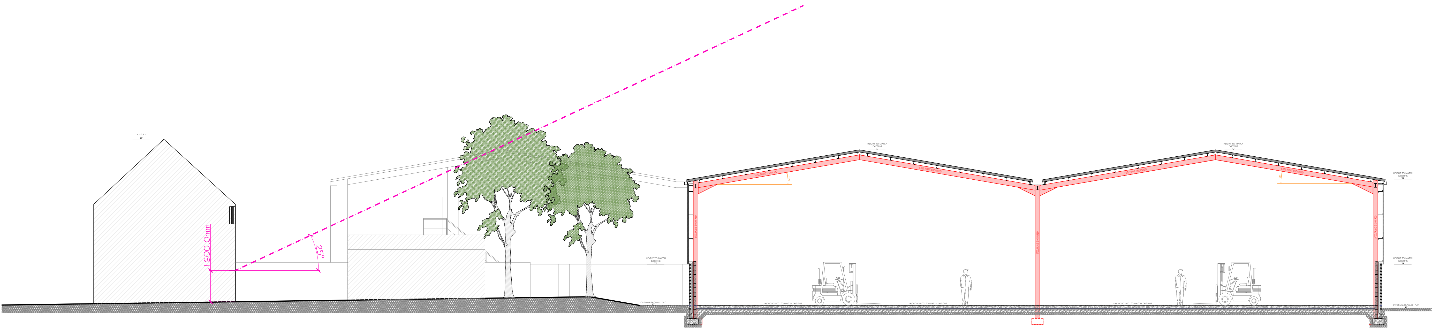
Proposed Cross Section A-A
