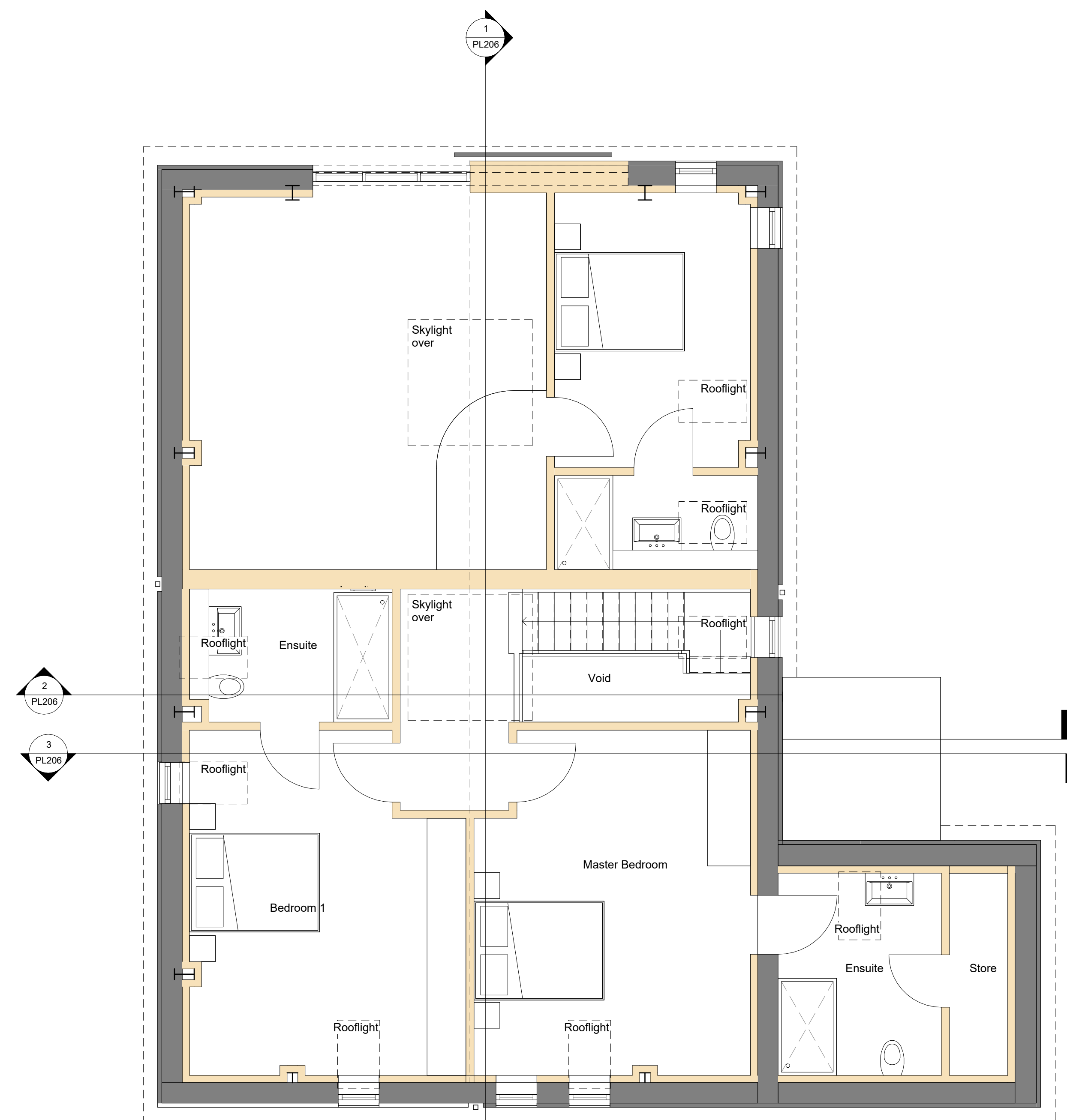
2 First Floor 1 : 50
