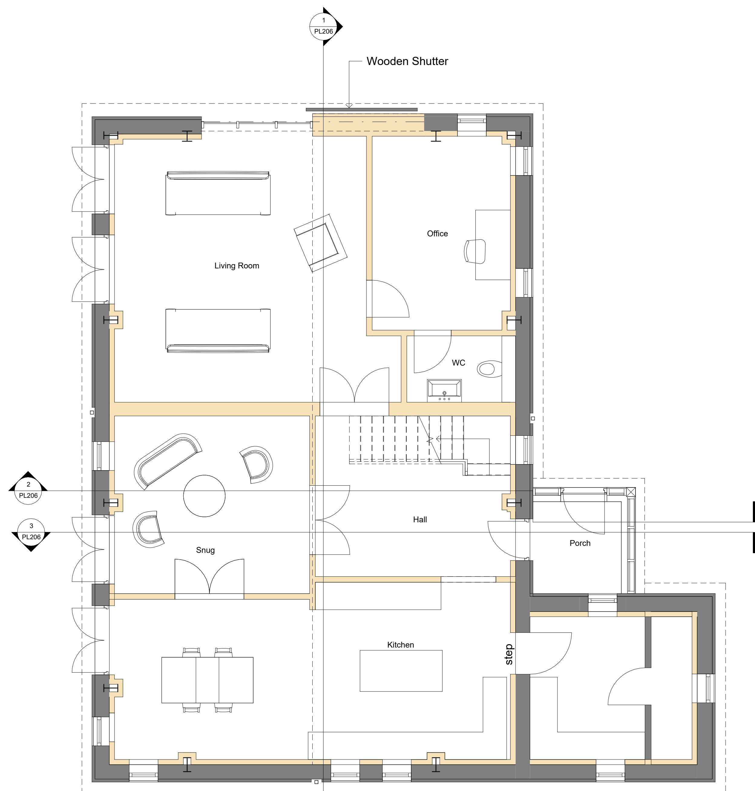
1 Ground Floor
