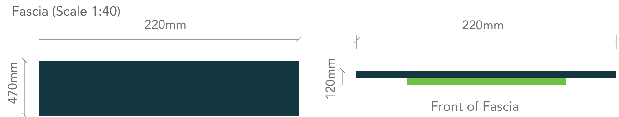
Plan View (1:40)
