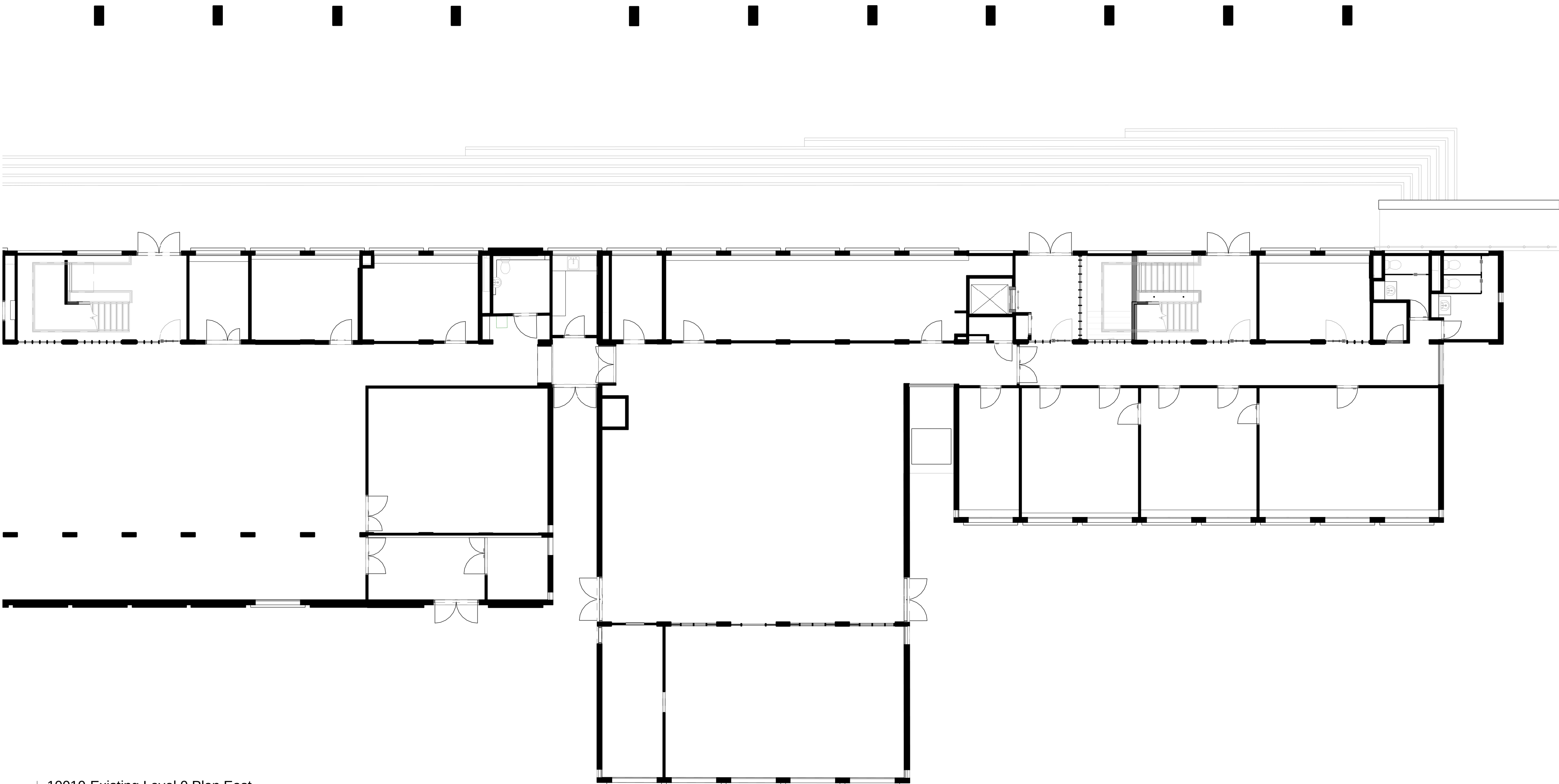
3 | 10010-Existing Level 0 Plan East 1 : 100
