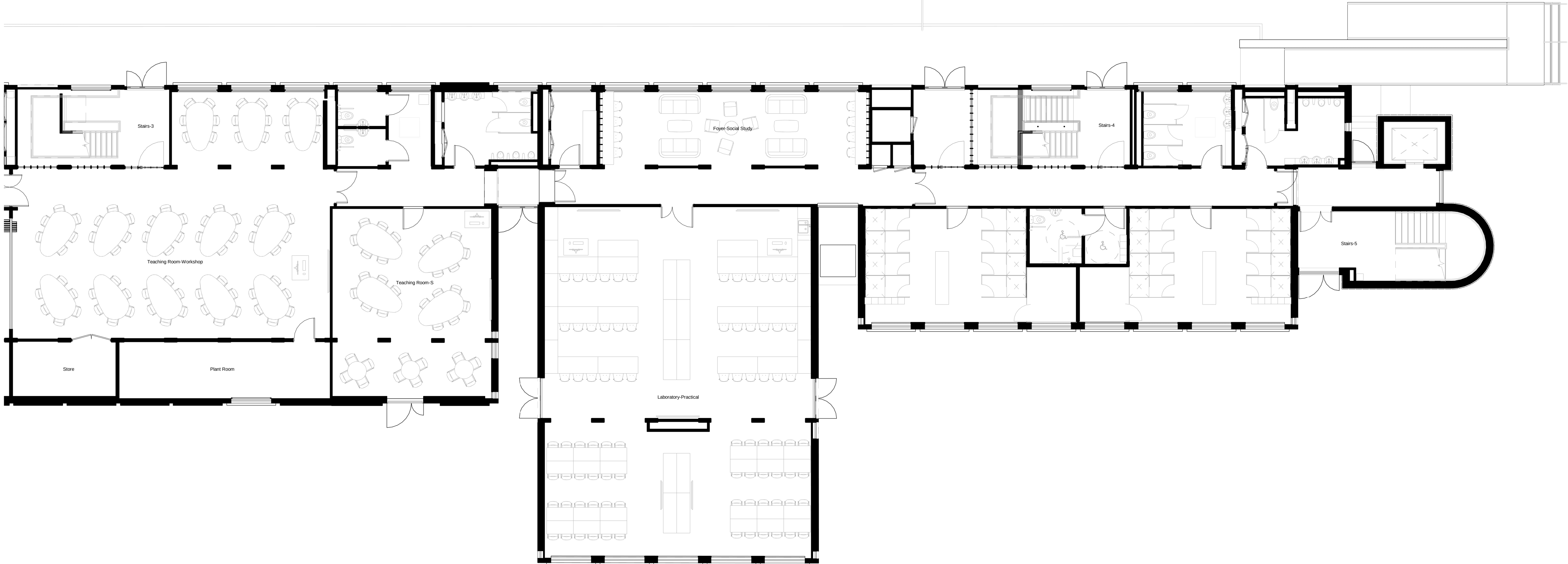
3 | 10310-Level 0 Plan East 1 : 100
