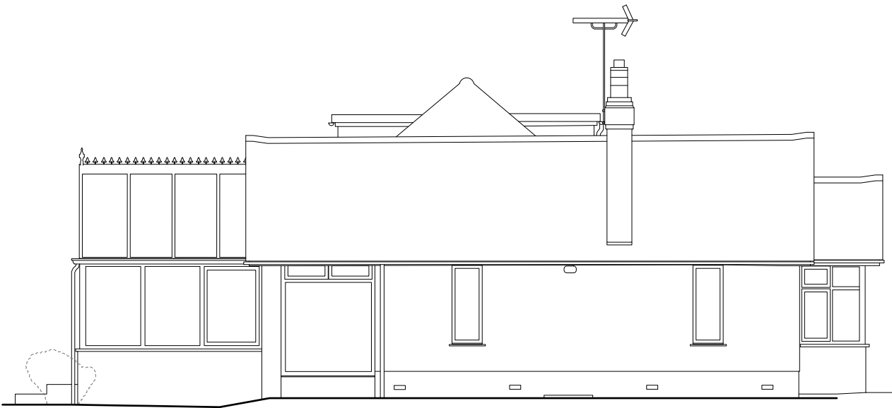
4 East Elevation
