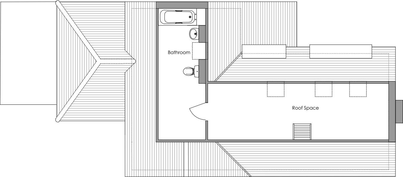
Existing Second Floor Plan
