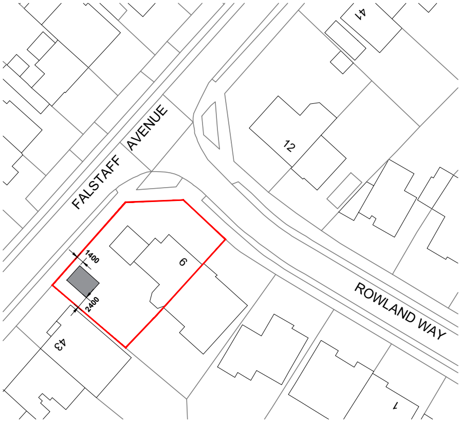
Block Plan 1:500
