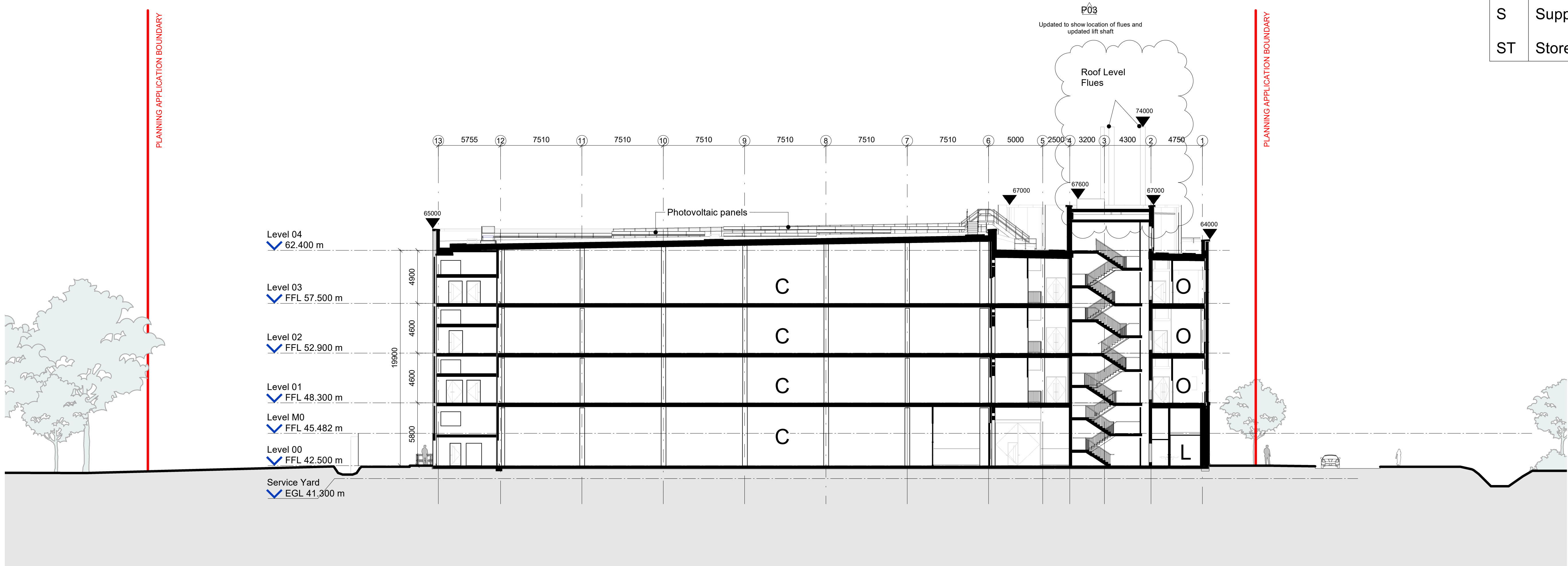
1 Section F-F 1 : 200 0 4 8 m Scale 1:200
