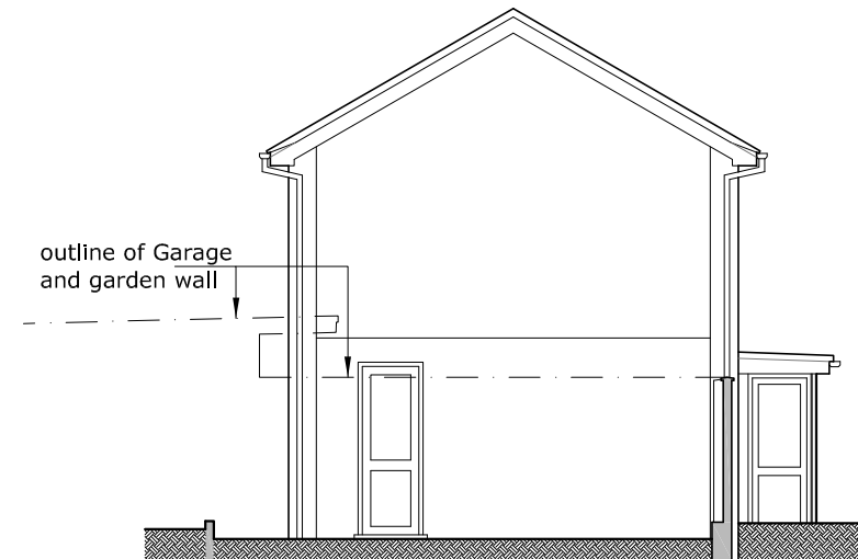
Existing West (Side) Elevation
