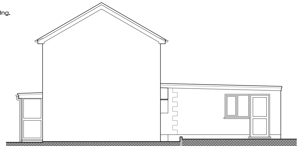
Proposed East (Side) Elevation (no change)
