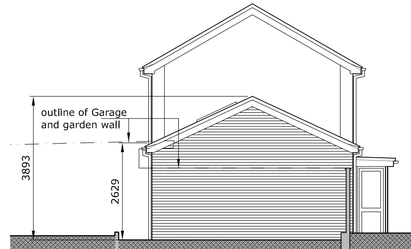
Proposed West (Side) Elevation
