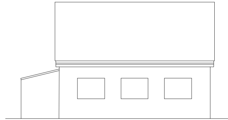
Side Elevation 1 :100 Garage
