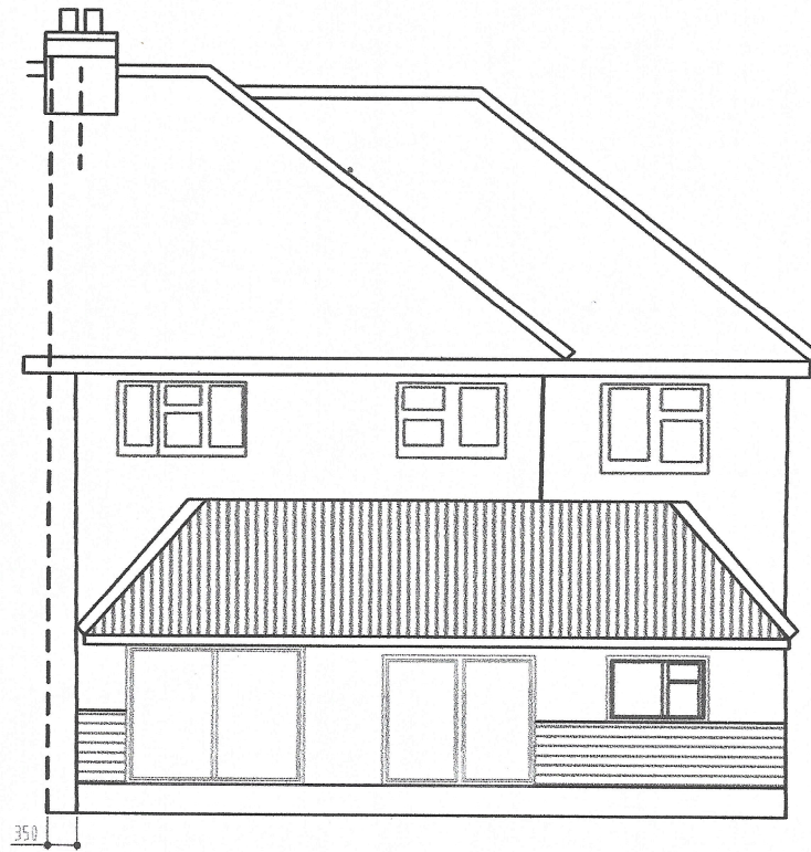
REAR ELEVATION AS EXISTING SCALE 1:100
