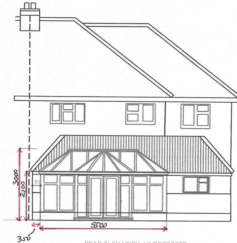
REAR ELEVATION AS PROPOSED SCALE 1:100
