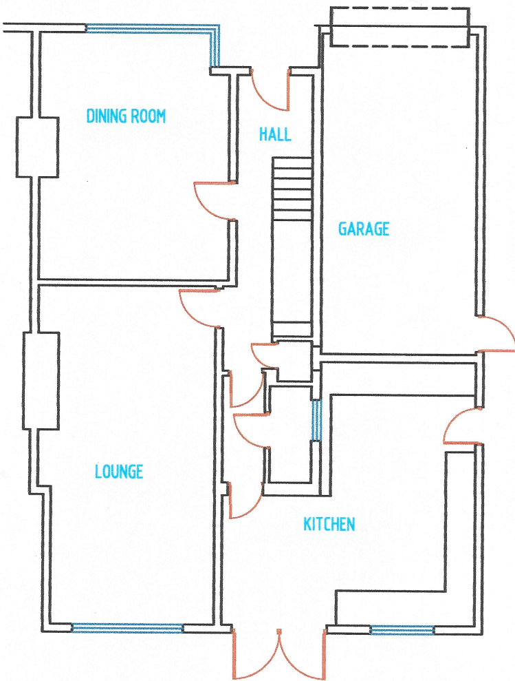
GROUND FLOOR PLAN AS EXISTING SCALE 1:100
