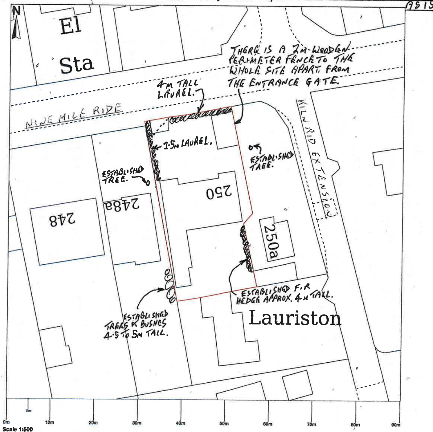
Fig. 1 250 Nine Mile Ride, Finchampstead, Wokingham, RG40 3PA IDENTIFYING PERIMETER OF SITE, FENCING, TREES & HEDGES ALL TO REMAIN
