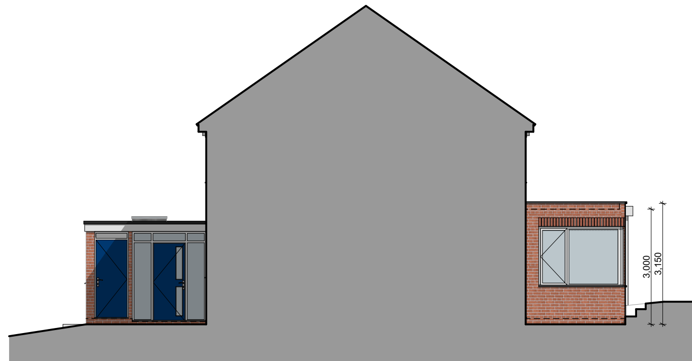
4 Side Elevation 1:100
